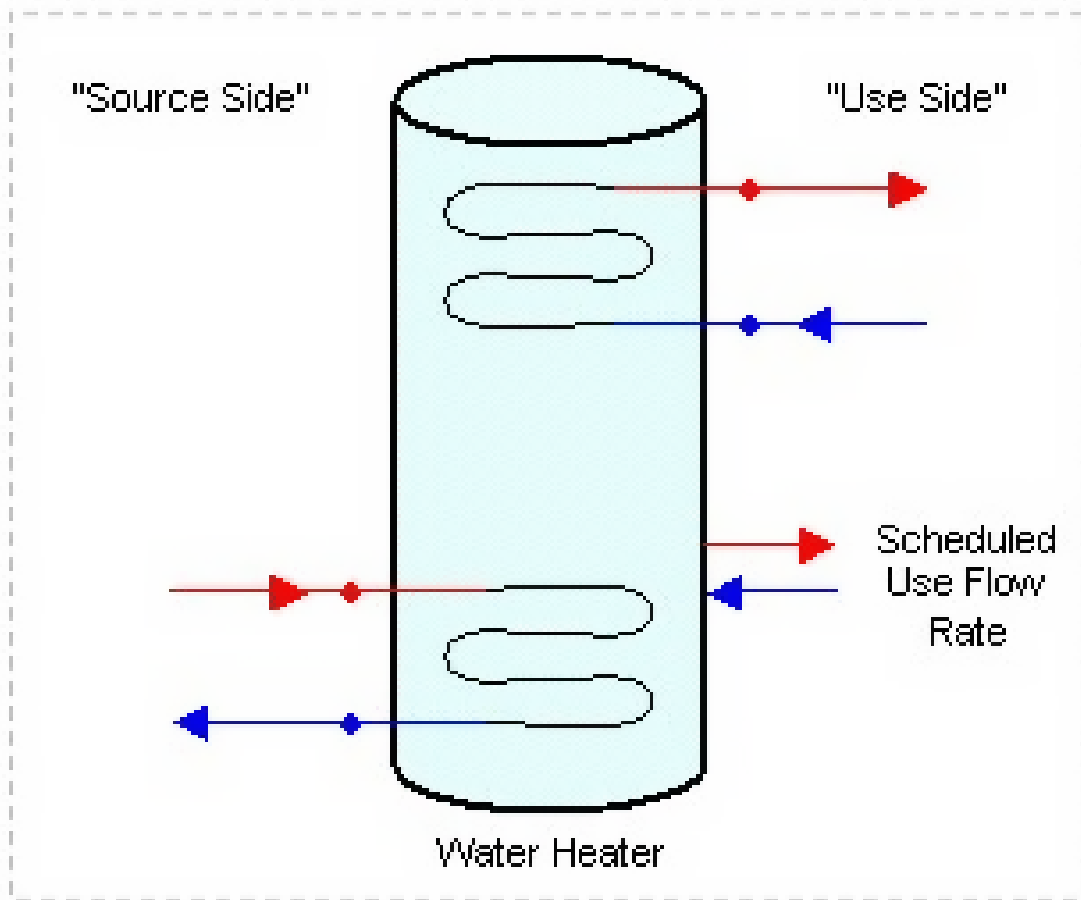
Figure 1.97: Water Heater Configuration
