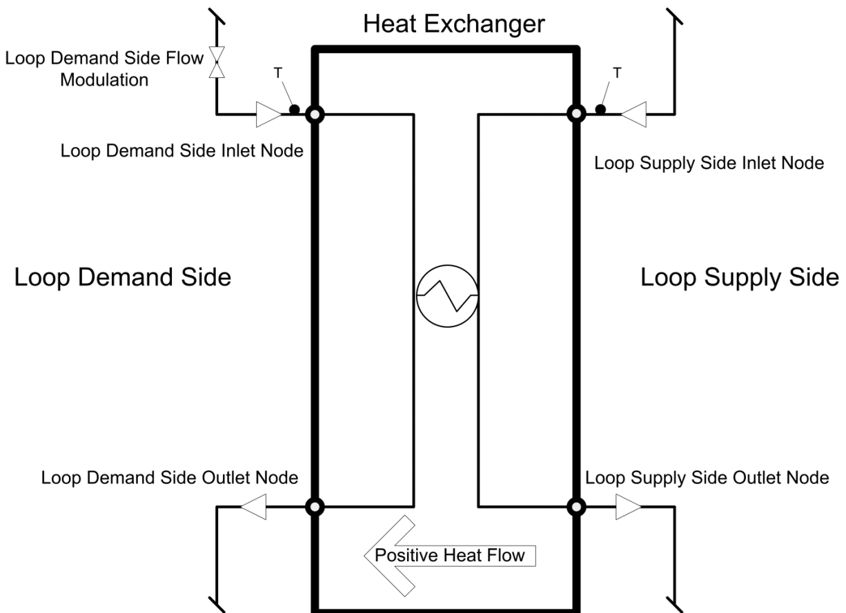
Figure 1.107: Plant Fluid-to-Fluid Heat Exchanger
