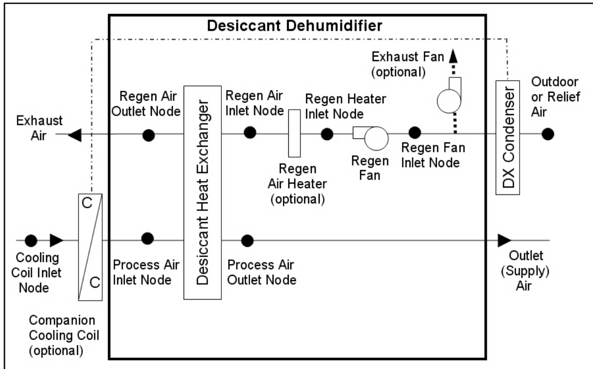
Figure 1.184: Schematic of Dehumidifier:Desiccant:System with Blow Through Regeneration Fan Placement
