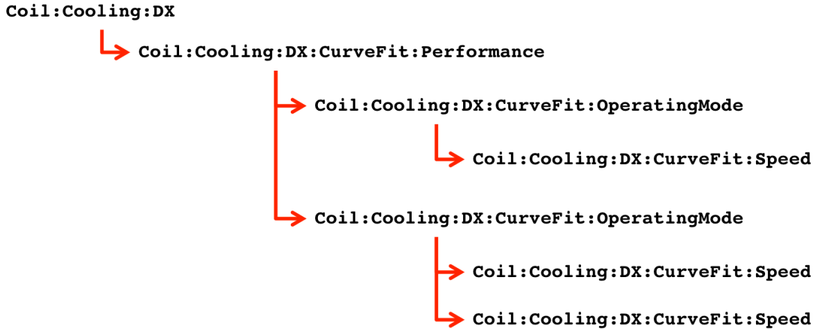
Figure 1.182: Hierarchy of references between cooling coil objects
