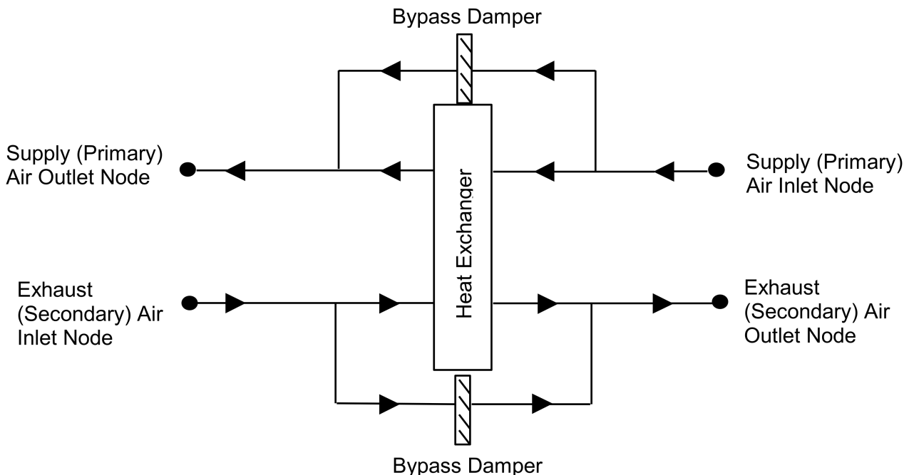
Figure 1.192: Schematic of the Sensible and Latent Air-to-Air Heat Exchanger
