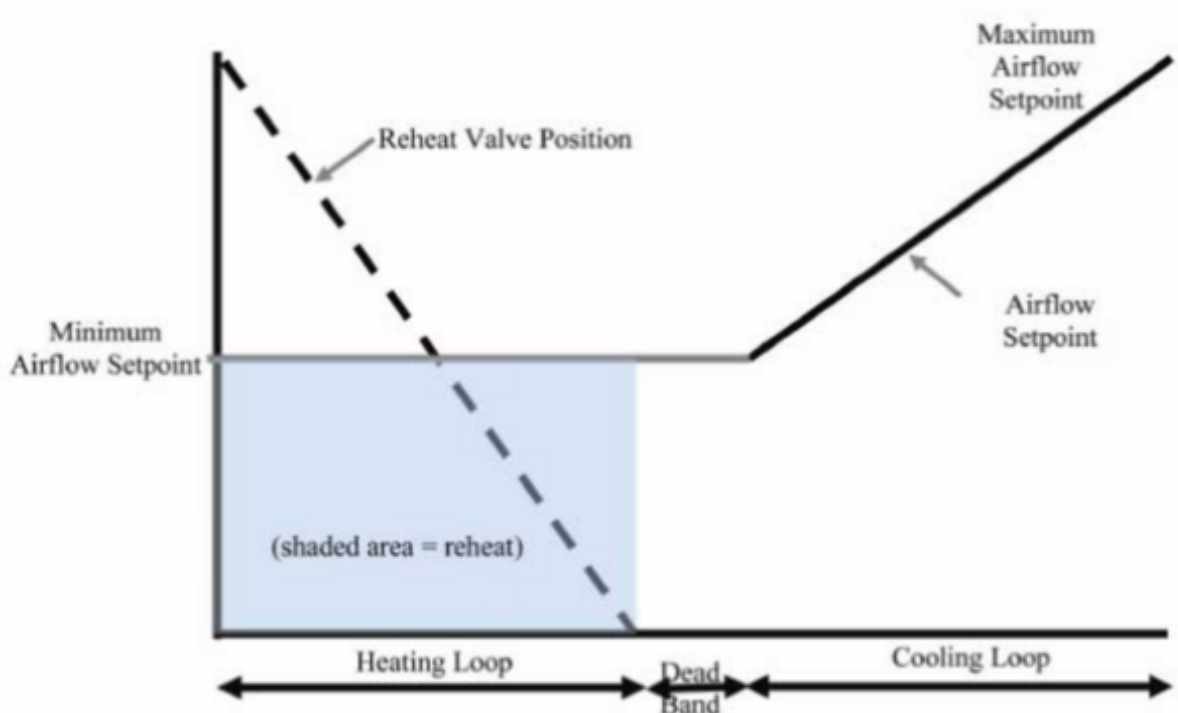
Figure 1.123: The Single Maximum Control Logic
