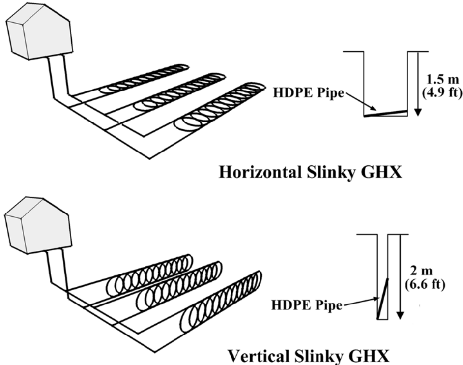
Figure 1.101: slinky heat exchanger
