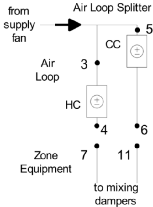
Figure 1.121: Air Loop/Zone Equipment Node Diagram
