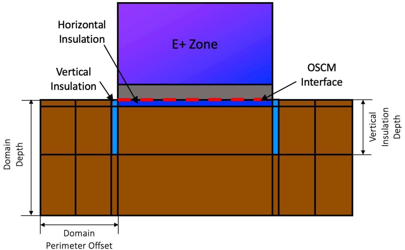
Figure 1.8: On-grade configuration
