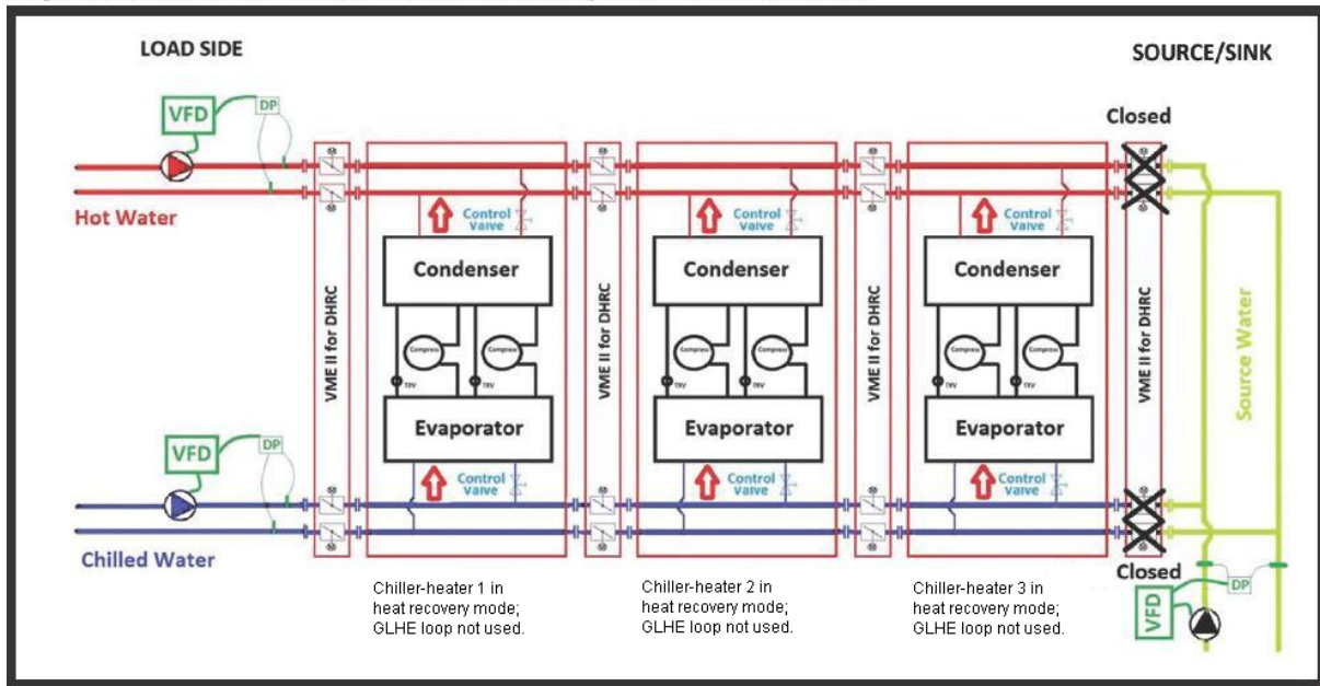
Diagram of Chiller-Heater bank with all modules in heat recovery mode, no GLHE water used.
