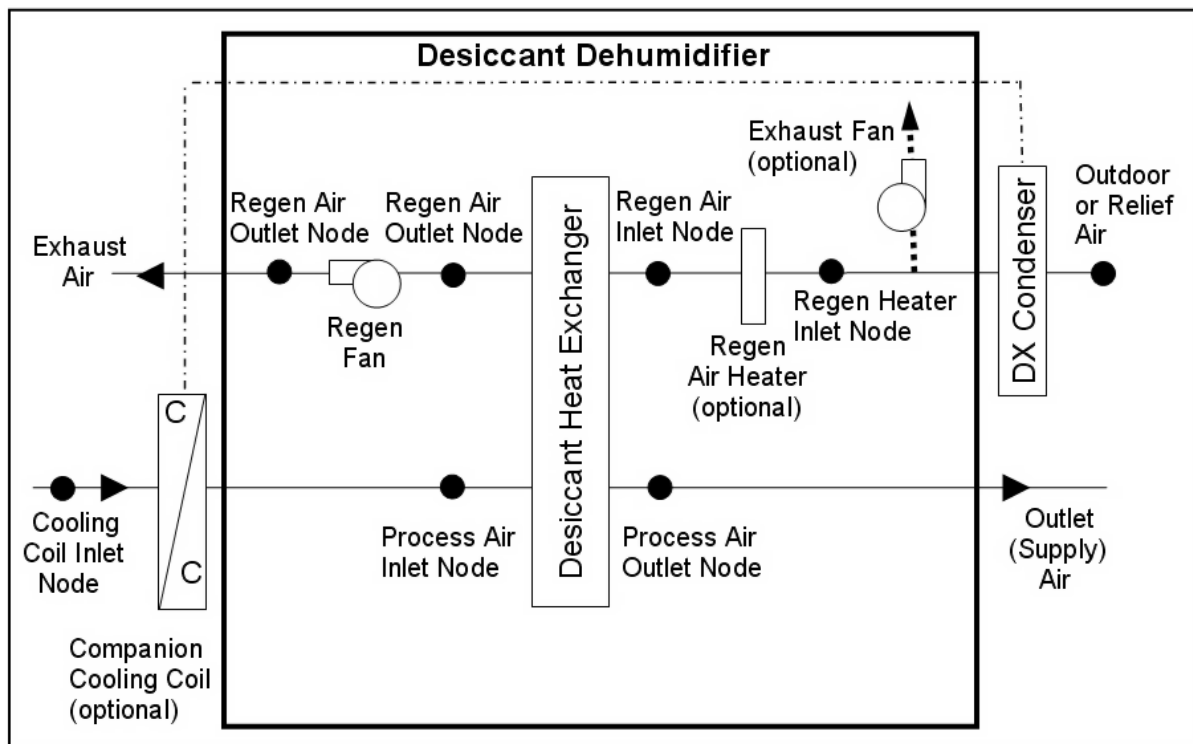
Figure 1.183: Schematic of Dehumidifier:Desiccant:System with Draw Through Regeneration Fan Placement
