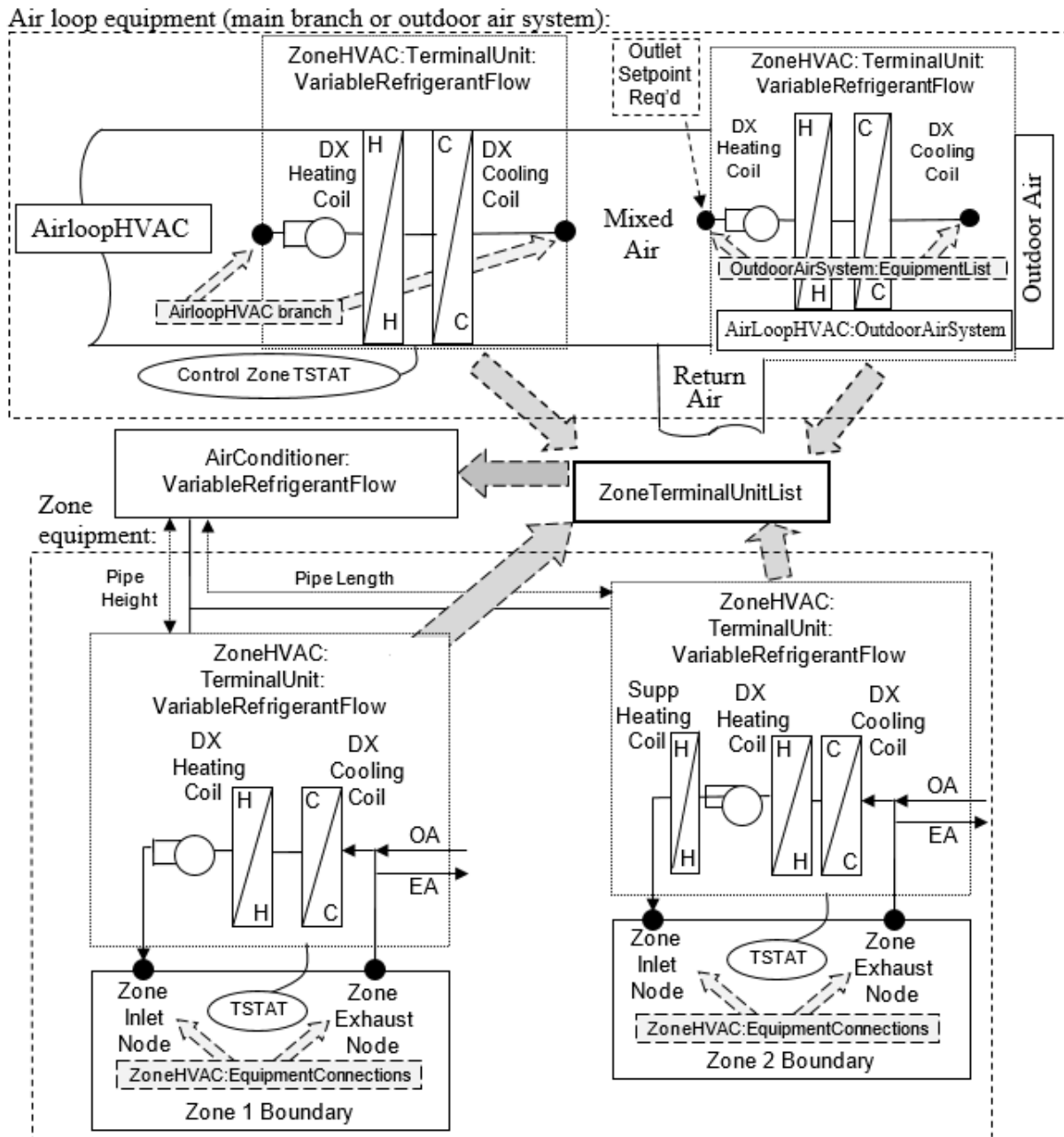
Figure 1.160: Variable Refrigerant Flow Schematic
