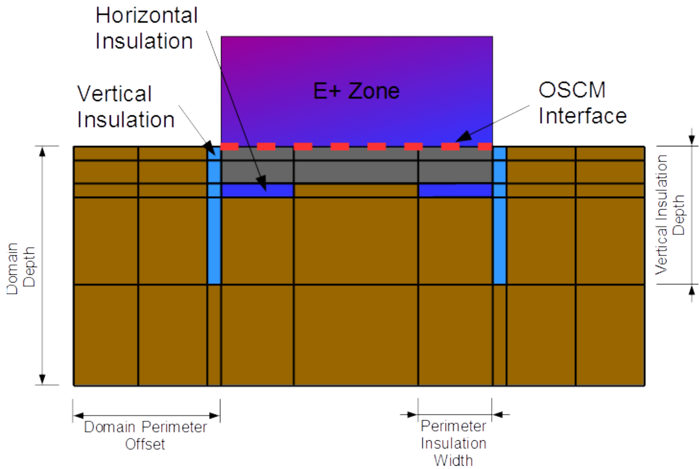
Figure 1.7: In-grade configuration.
