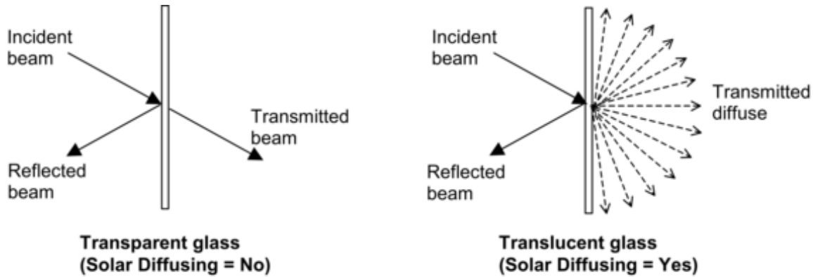
Figure 1.12: Comparison between transmittance properties of transparent glass (Solar Diffusing = No) and translucent glass (Solar Diffusing = Yes).
