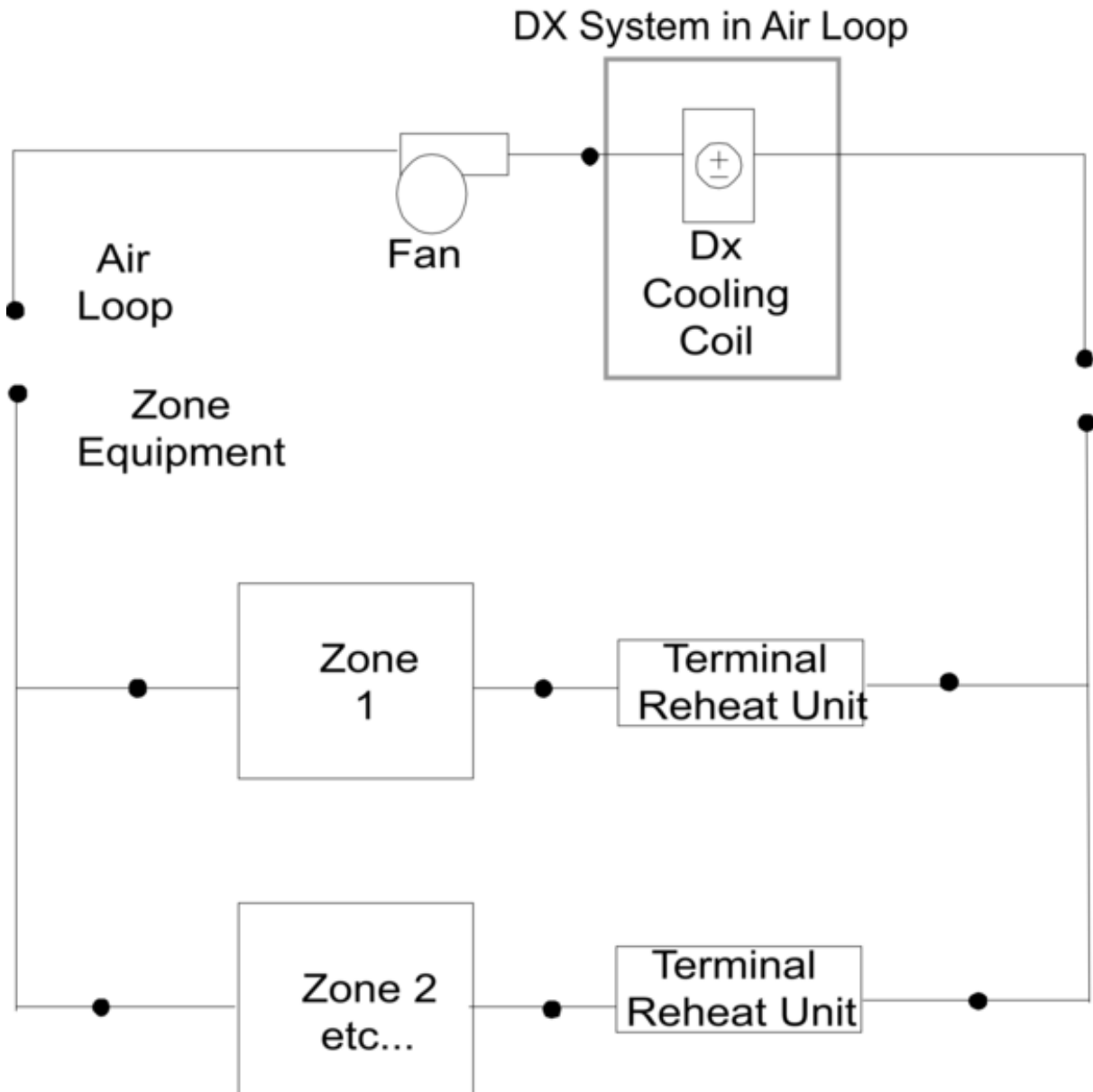
Figure 1.178: Schematic of CoilSystem:Cooling:DX Object in an Air Loop for a Blow Through Application
