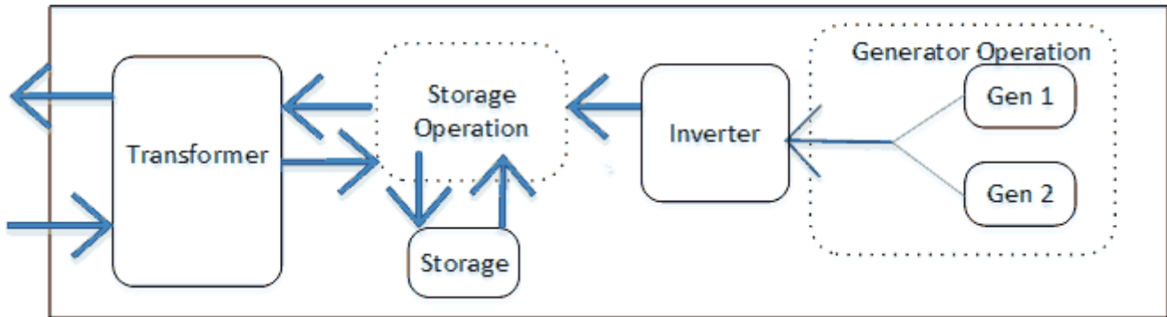
Figure 1.199: LoadCenterBusType
