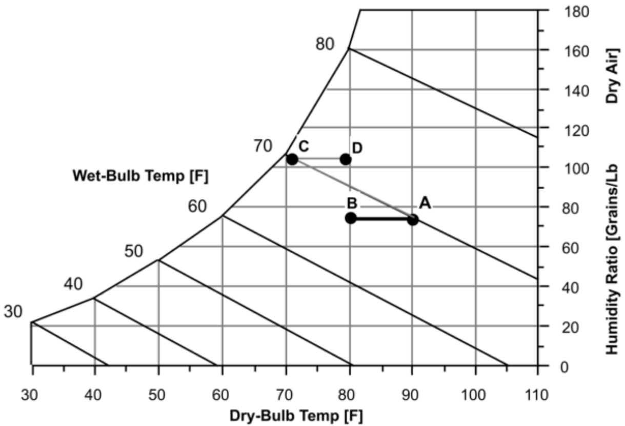
Figure 1.189: Secondary Air Process – Indirect Dry Coil Evap Cooler
