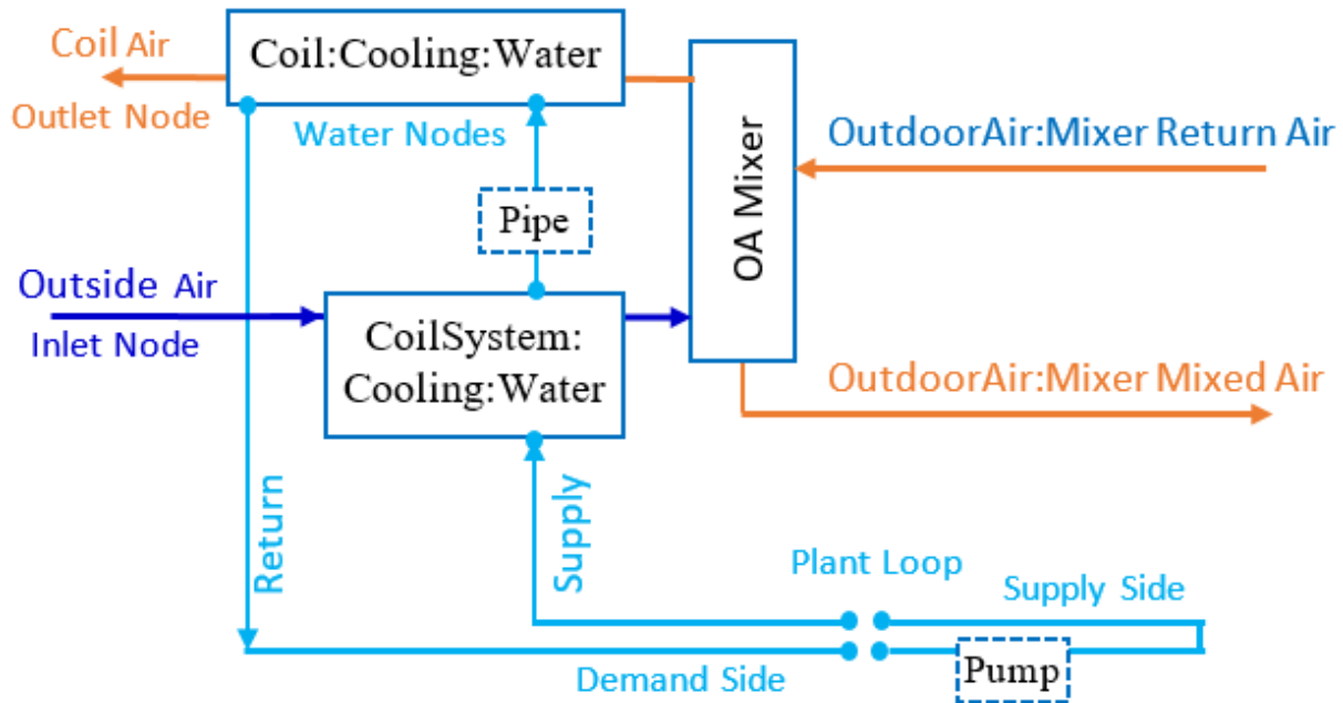
Figure 1.177: Wrap-Around Water Coil Heat Recovery System In Outdoor Air System
