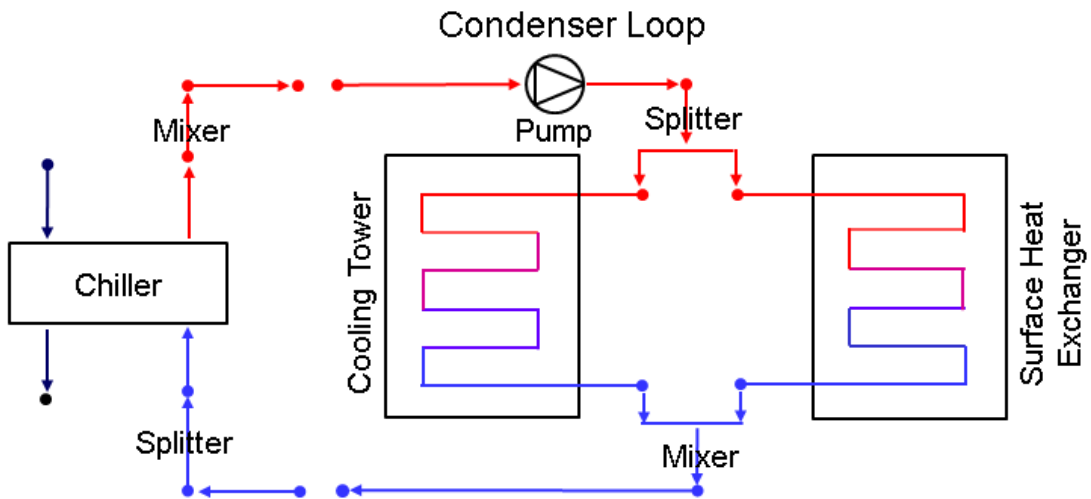
Figure 1.106: Surface Ground Heat Exchanger with other heat exchangers on condenser loop
