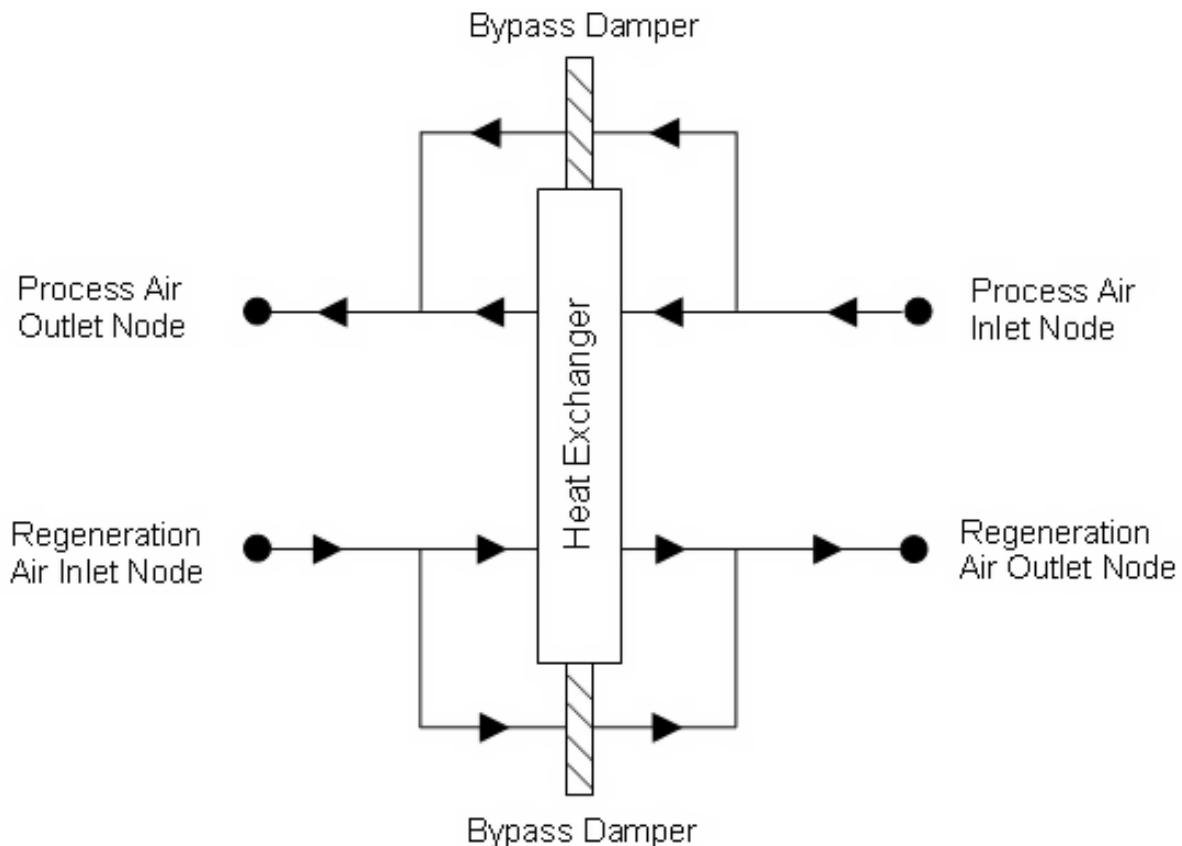
Figure 1.193: Schematic of the Balanced Flow Desiccant Heat Exchanger
