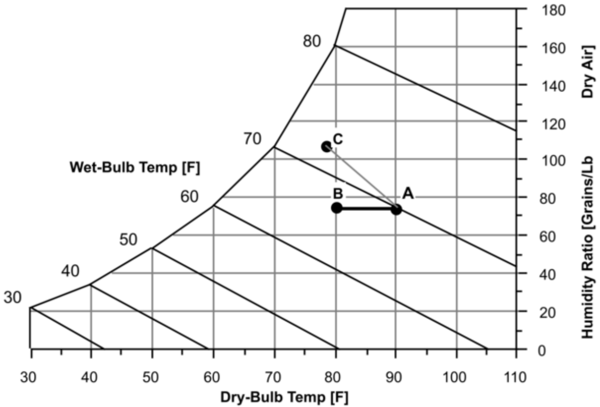
Figure 1.191: Secondary Air Process Indirect Wet Coil Evap Cooler
