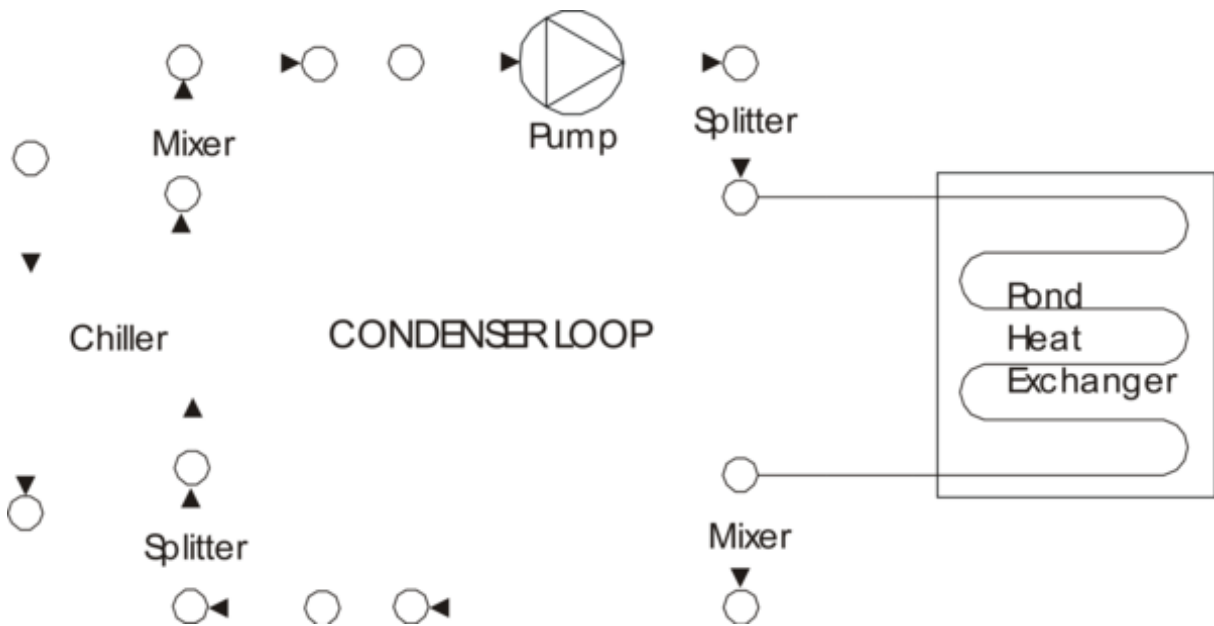
Figure 1.103: Example of Pond Ground Heat Exchanger as only heat exchanger on condenser loop
