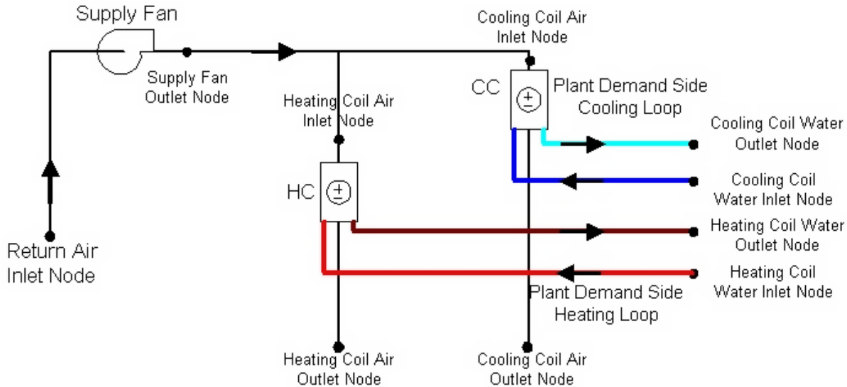
Figure 1.171: Example Air Loop Heating &amp; Cooling Coil
