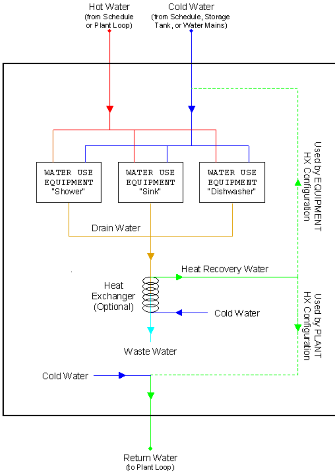
Figure 1.201: Diagram of internal connections for WaterUse:Connections
