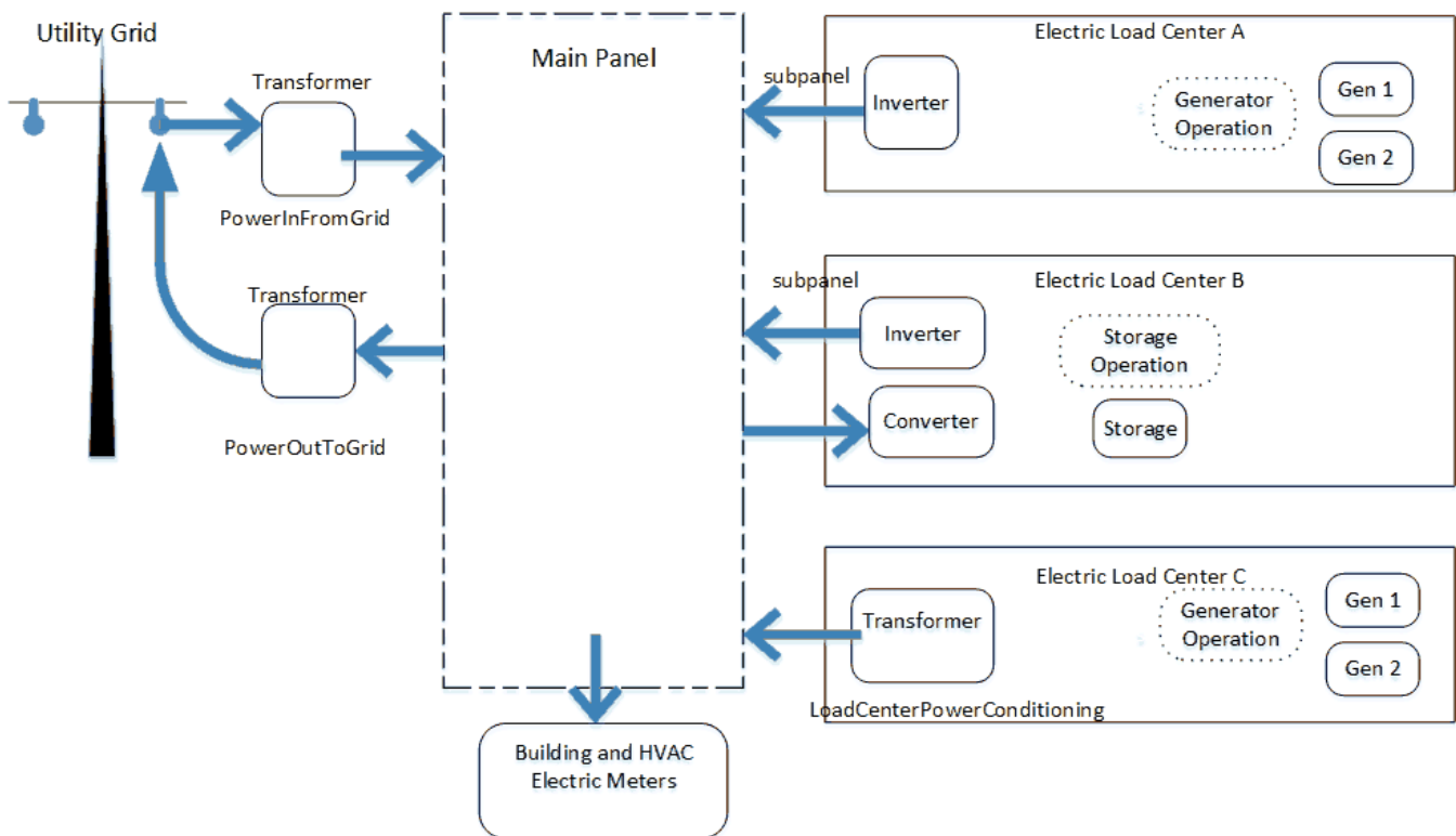
Figure 1.194: PowerServiceOverview
