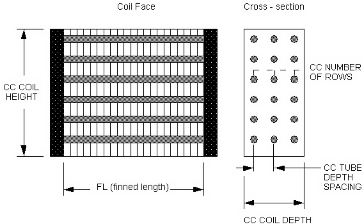
Figure 1.172: Geometry of a Cooling Coil (CC)
