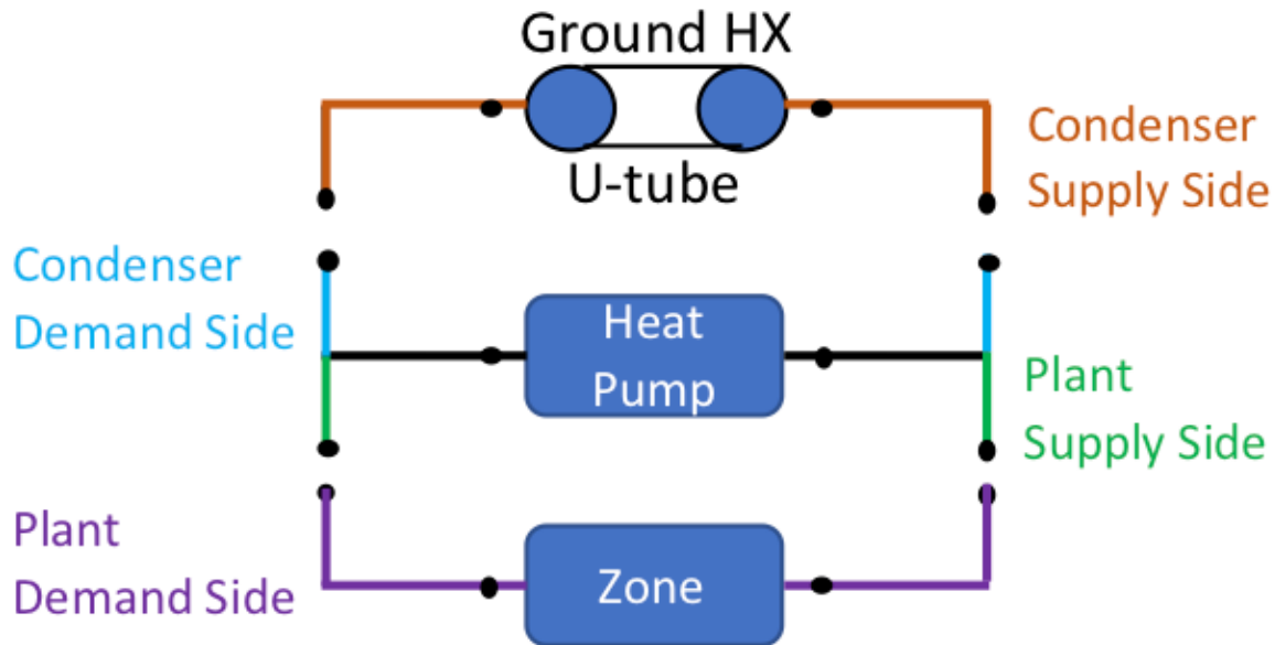
Figure 1.92: Schematic of EnergyPlus Ground Loop Heat Exchanger
