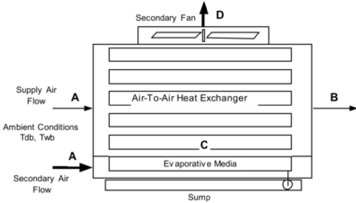
Figure 1.188: Evaporative Cooler – Indirect Dry Coil
