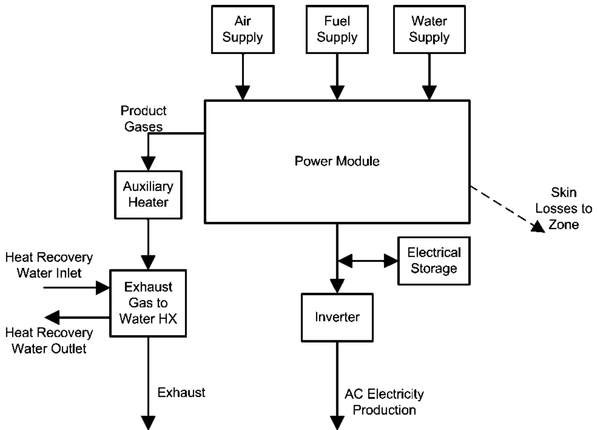
Figure 1.200: Fuel cell subsystems.
