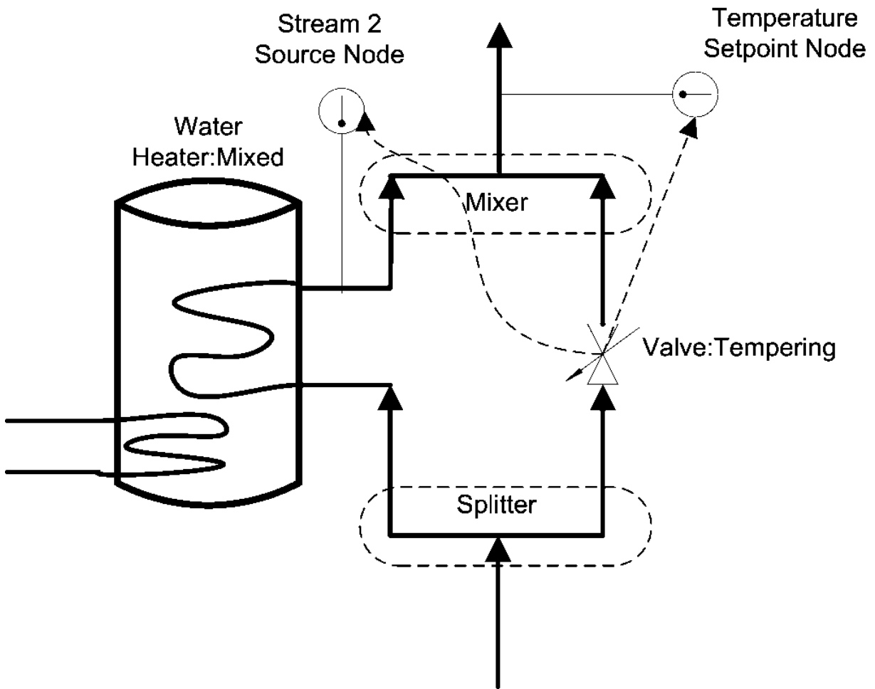
Figure 1.170: Tempering Valve Schematic
