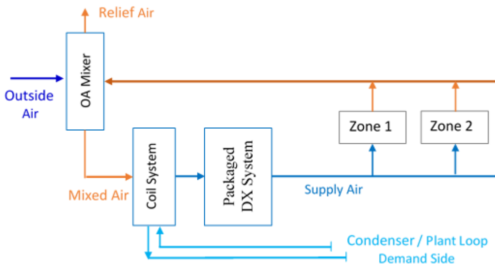
Figure 1.175: Water Side Economizer Coil System Upstream of Packaged DX System
