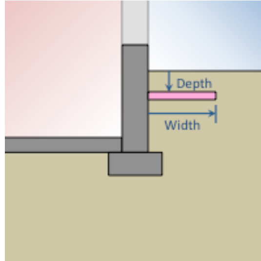
Figure 1.54: Placement of exterior horizontal insulation
