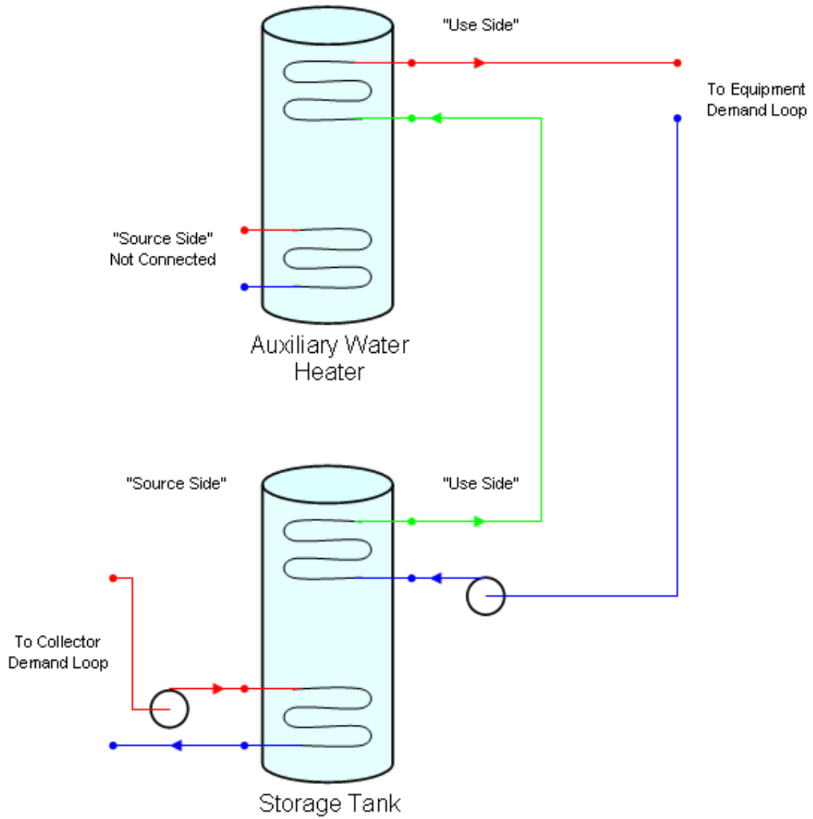
Figure 1.168: Two-Tank Solar Heating System Connection Diagram
