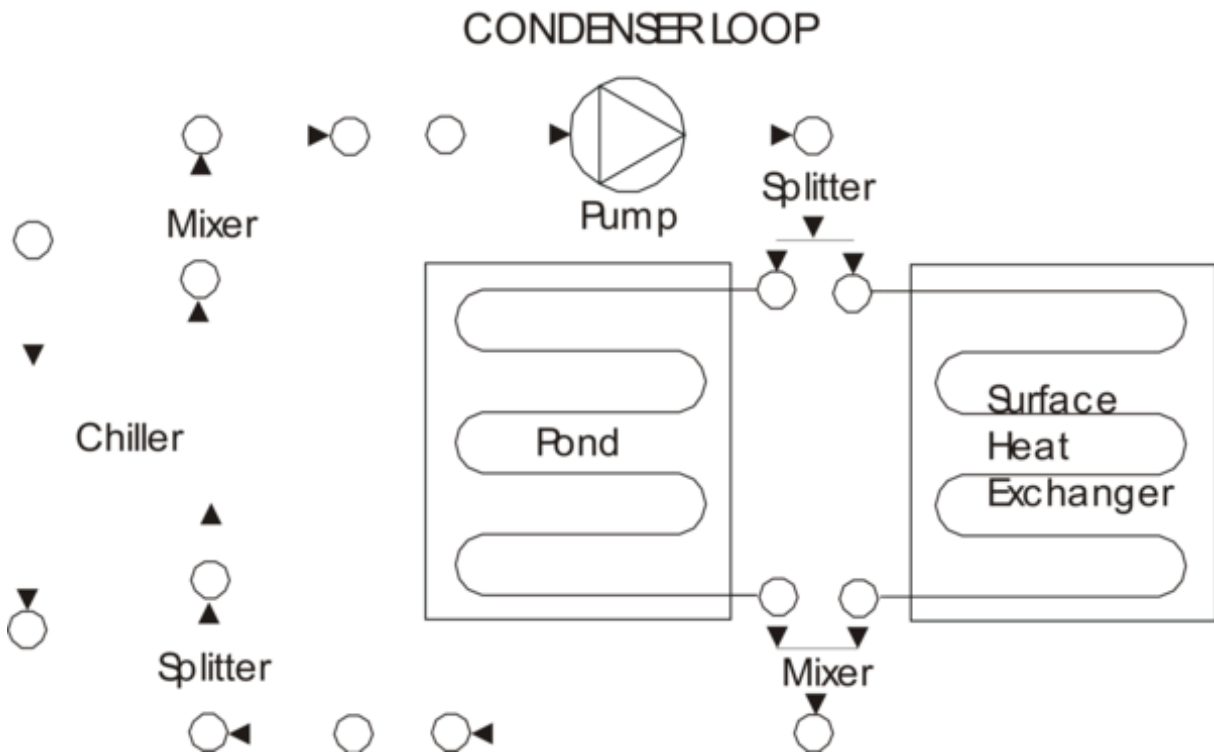
Figure 1.104: Pond Ground Heat Exchanger with other heat exchangers on condenser loop
