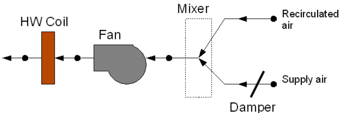
Figure 2.6: Series PIU Terminal Unit
