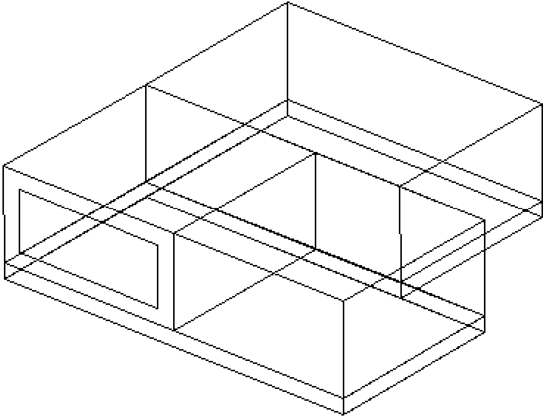
Figure 1.166: Illustration of AirLoopHVAC:SupplyPlenum
