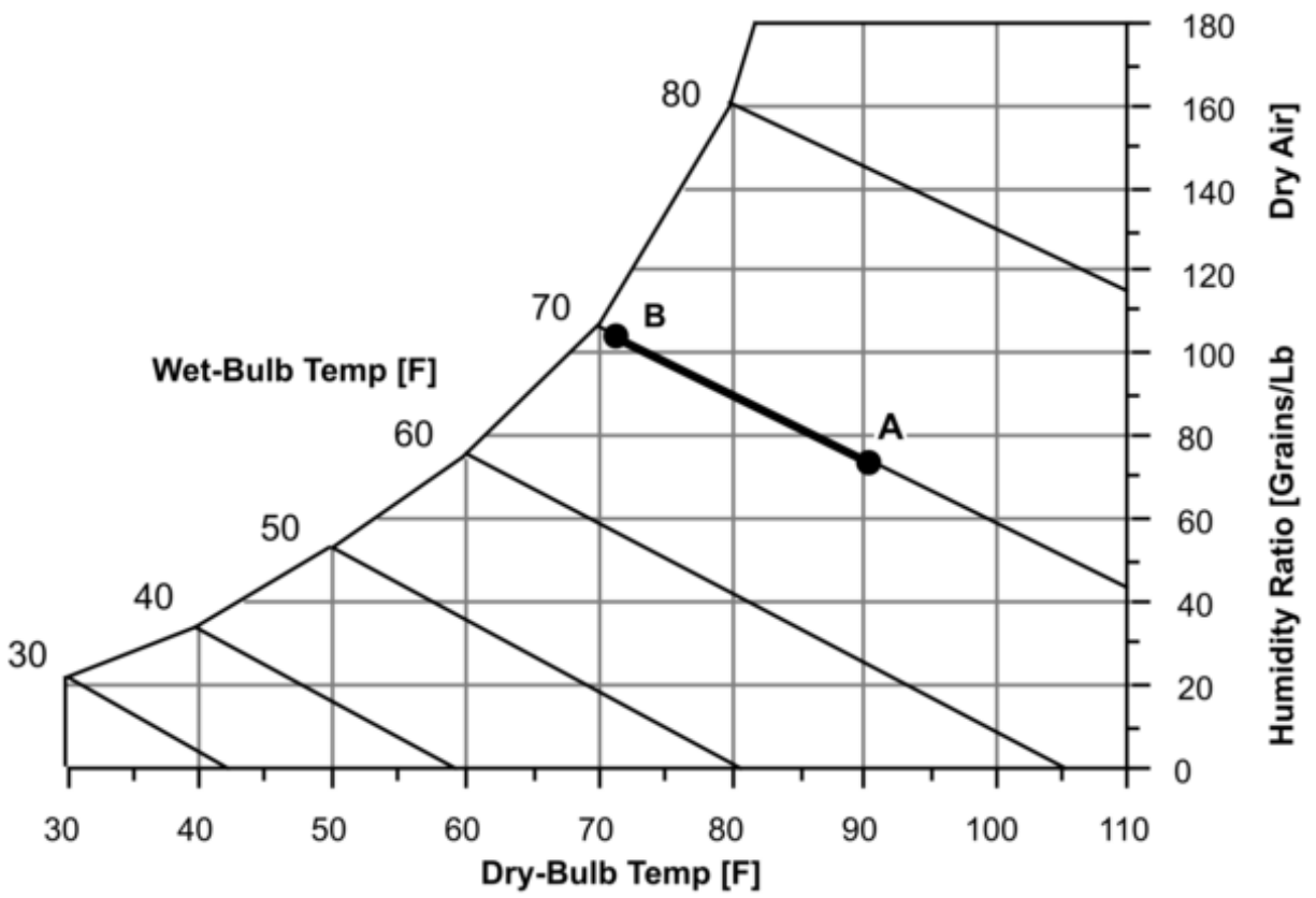
Figure 1.187: Psychrometric Chart – Constant Enthalpy
