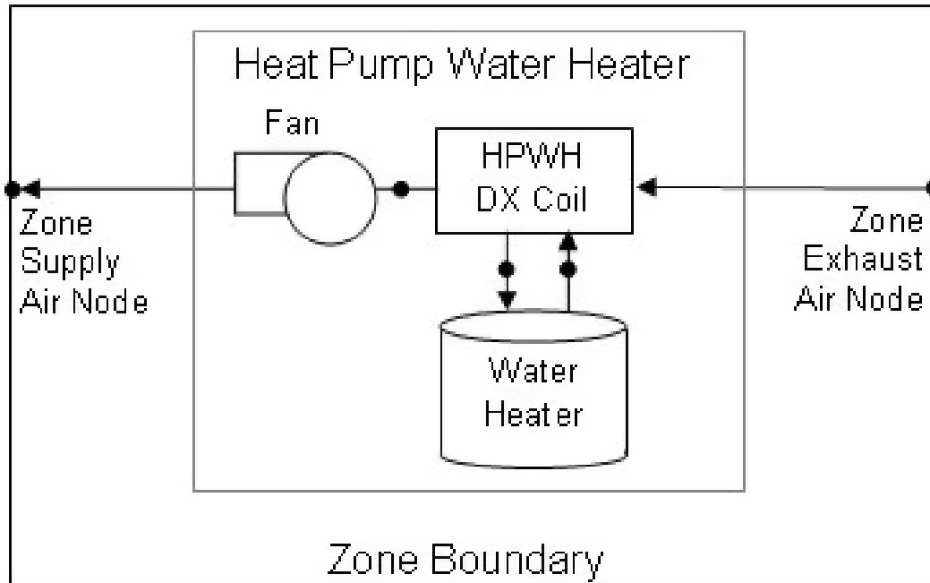
Figure 1.98: Schematic diagram for a heat pump water heater located in a zone
