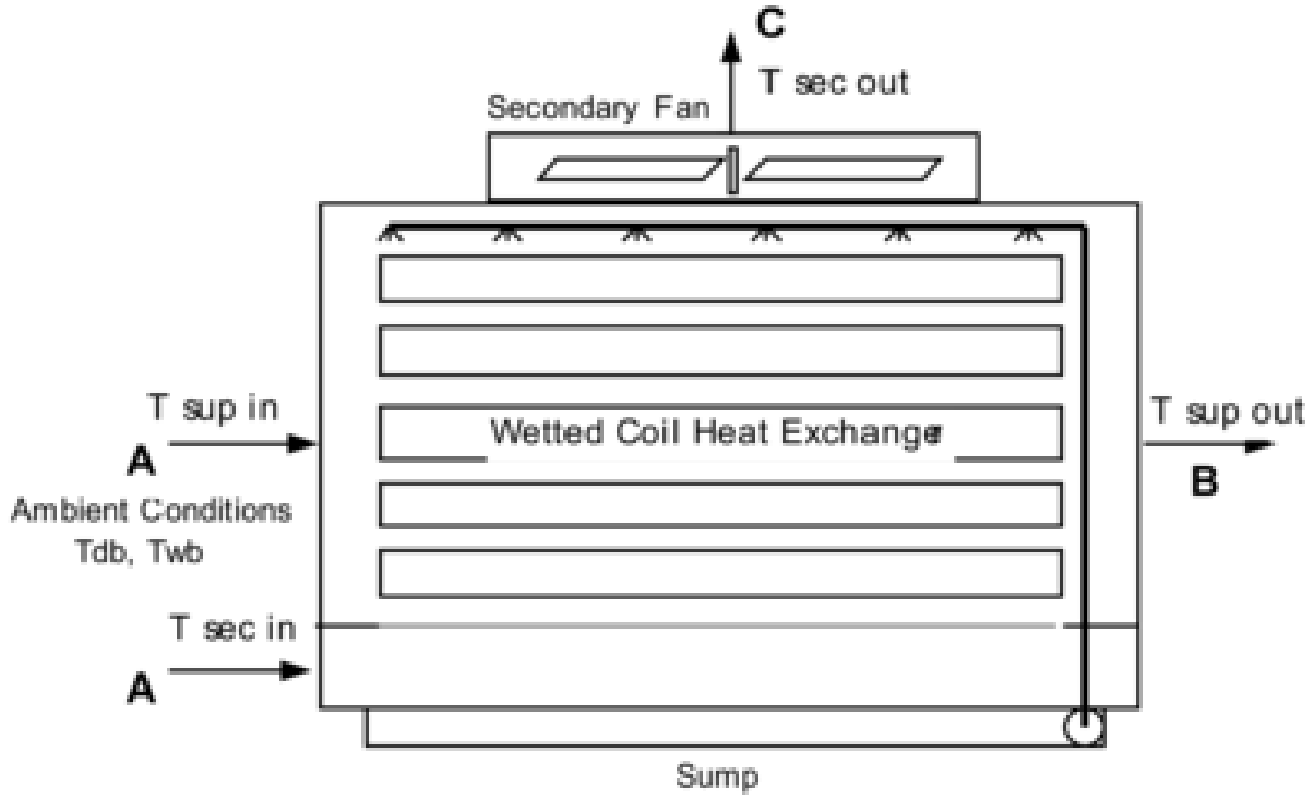
Figure 1.190: Evaporative Cooler Indirect Wet Coil
