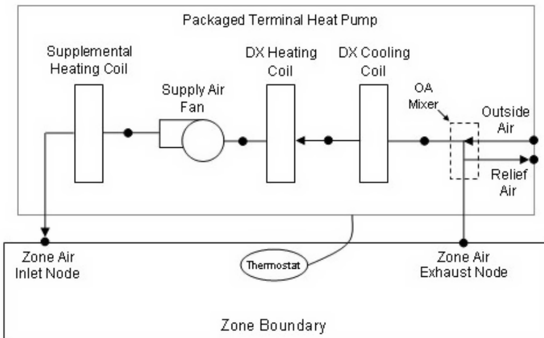
Figure 2.2: Schematic of a packaged terminal heat pump (draw through fan placement)
