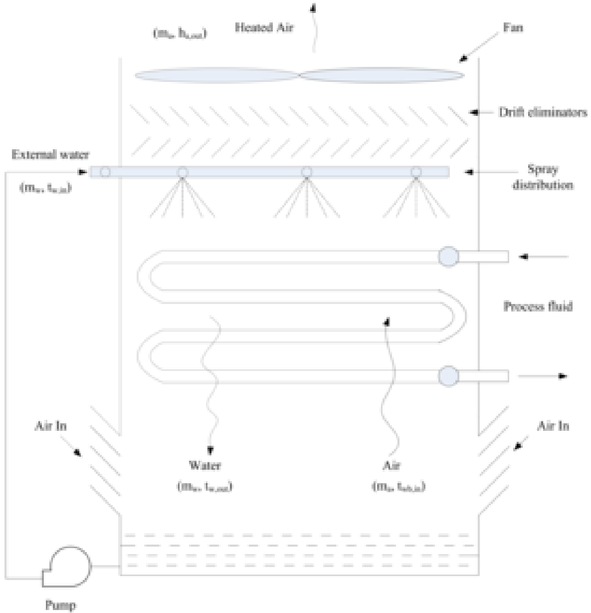
Figure 1.99: Schematic diagram for evaporative fluid cooler
