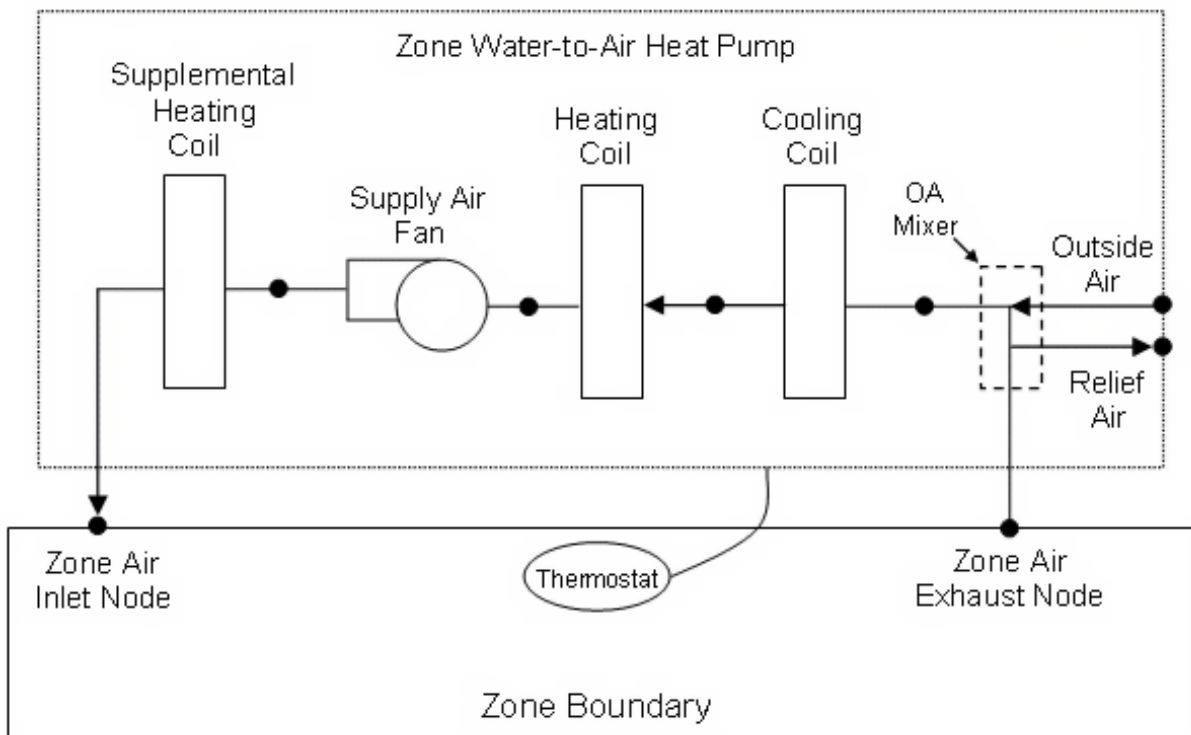
Figure 1.134: Zone Water to Air Heat Pump Schematic for a DrawThrough Configuration with Ground Heat Exchanger
