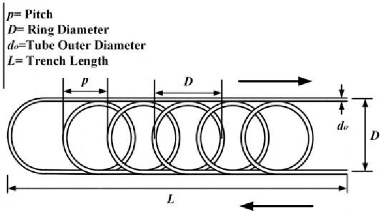
Figure 1.102: slinky heat exchanger
