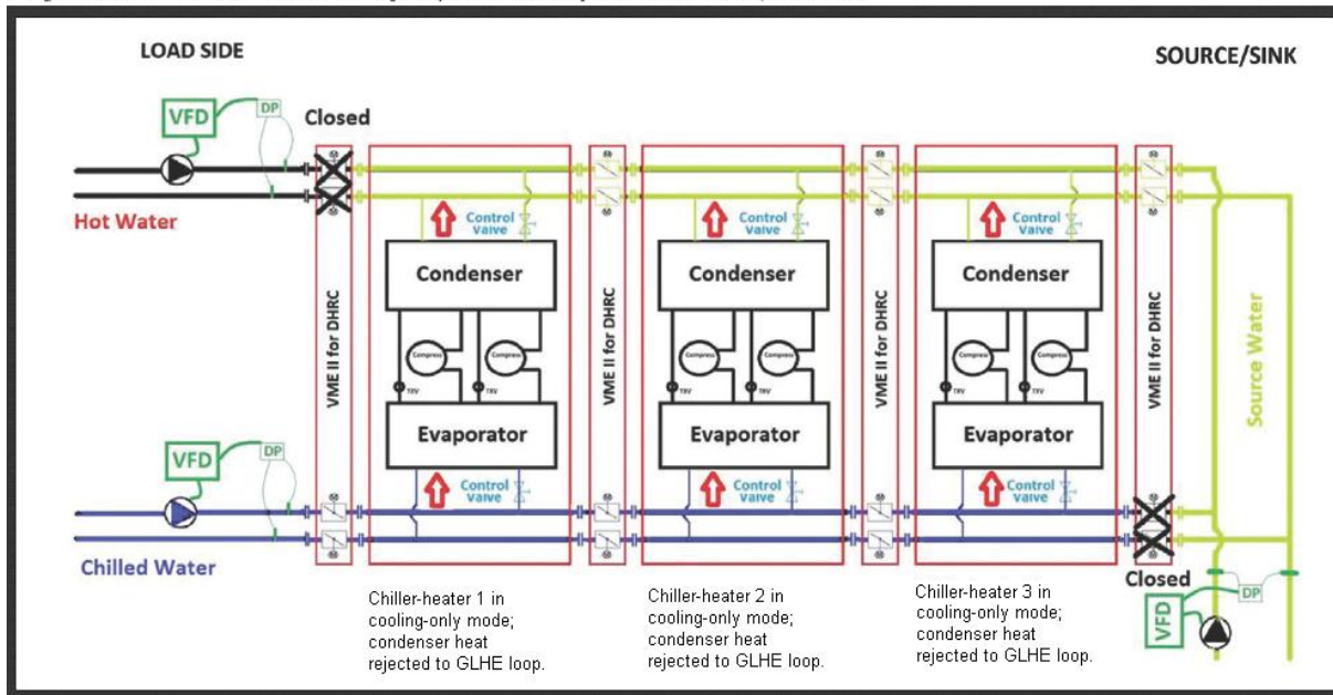
Diagram of chiller-heater bank in cooling-only mode, condenser heat rejected to GLHE loop.
