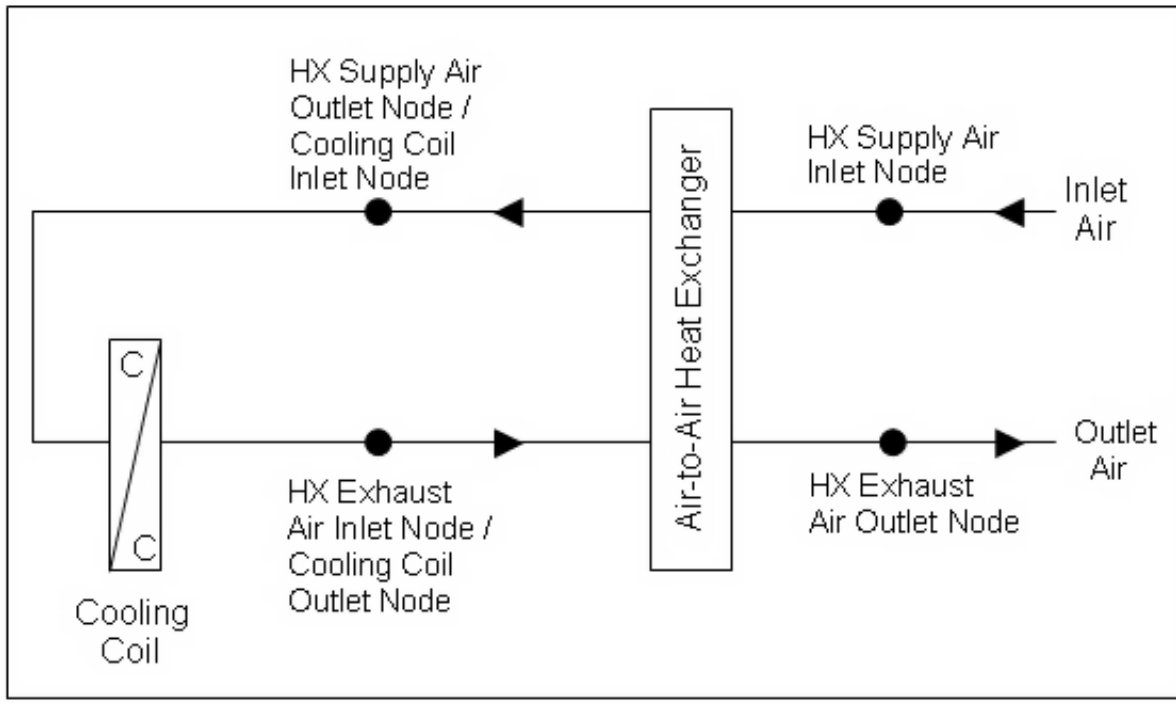
Figure 1.179: Schematic of the CoilSystem:Cooling:DX:HeatExchangerAssisted compound object
