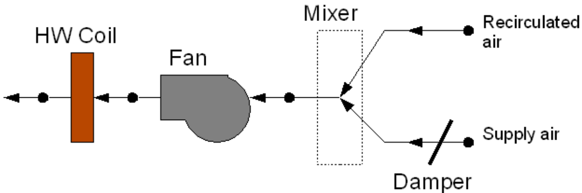
Figure 2.5: Series PIU Terminal Unit
