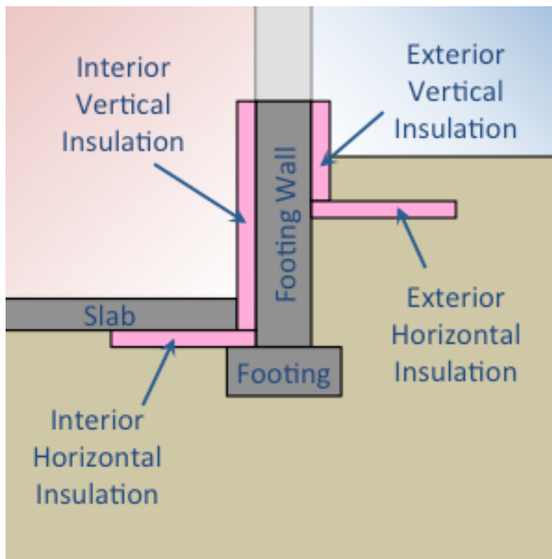
Figure 1.47: Structural and insulation components of Foundation:Kiva objects
