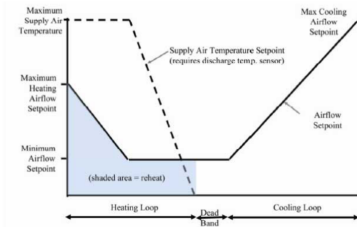
Figure 1.127: The Dual Maximum Control Logic
