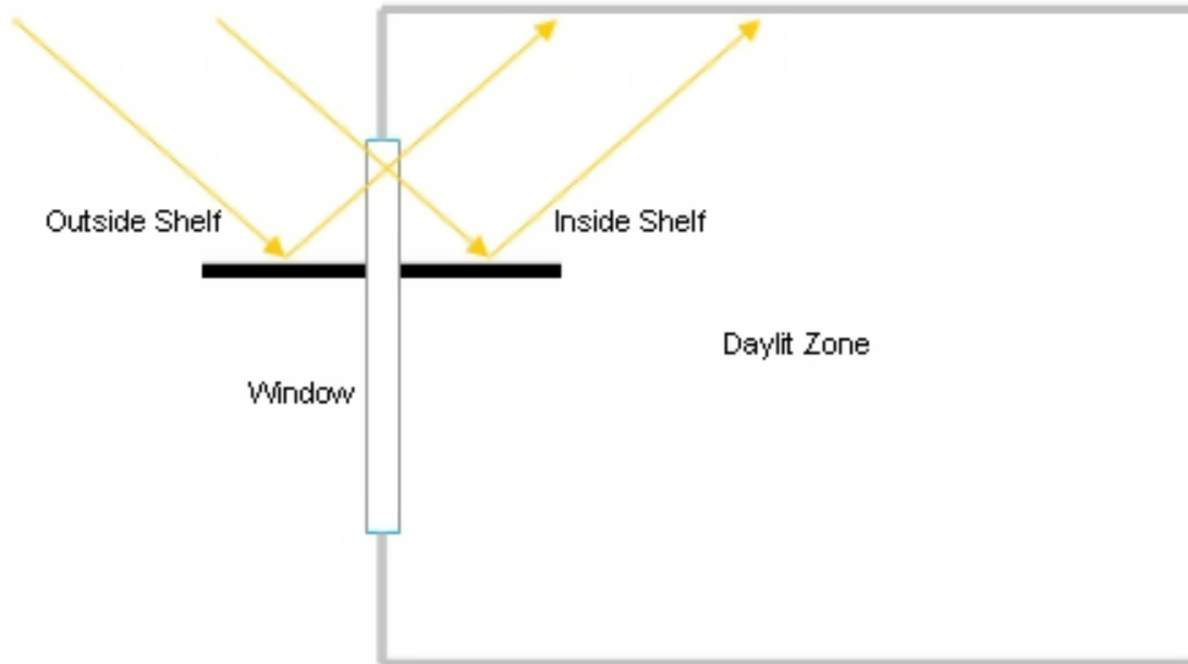
Figure 1.85: Daylighting shelf diagram.
