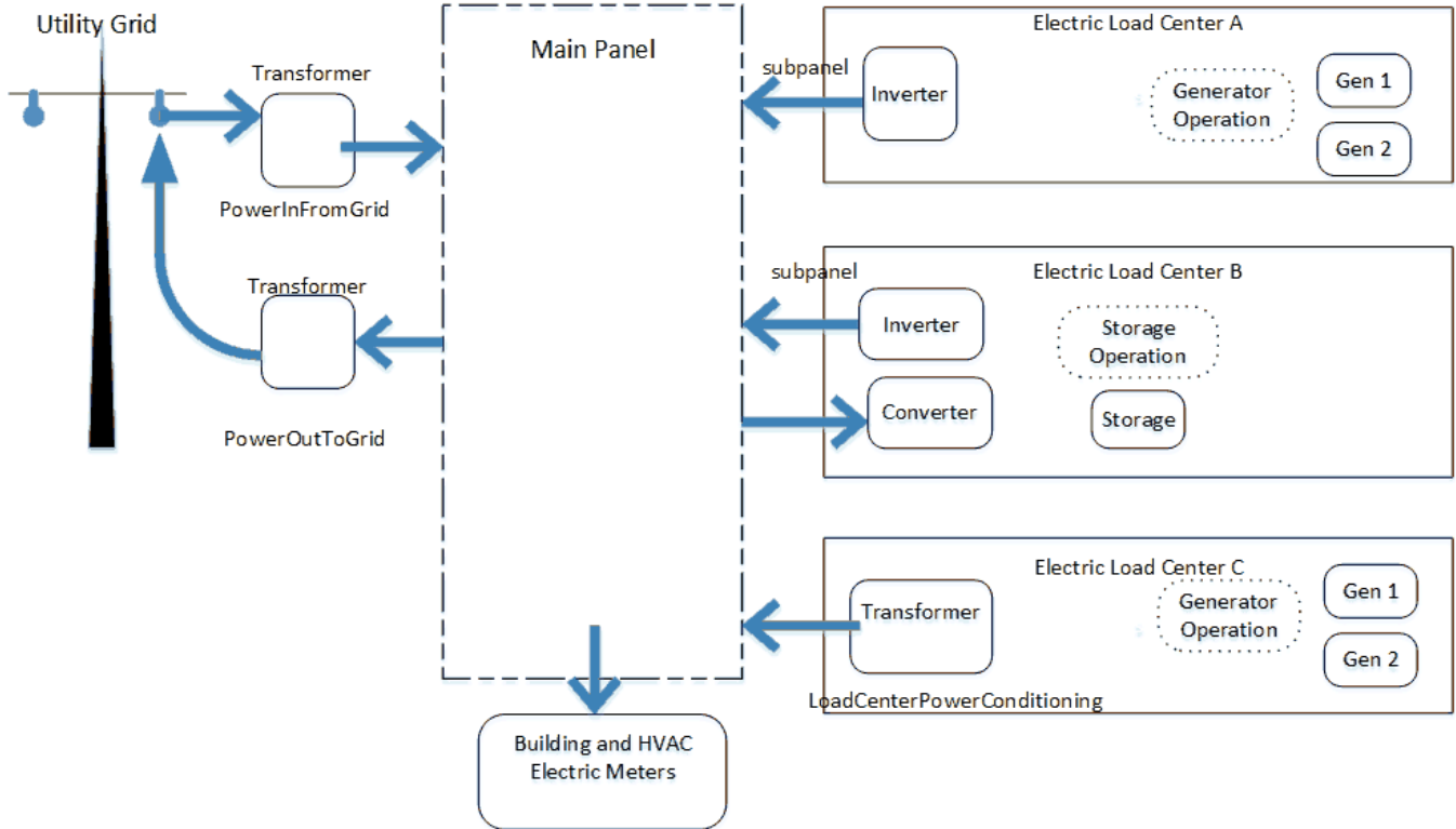
Figure 1.199: PowerServiceOverview
