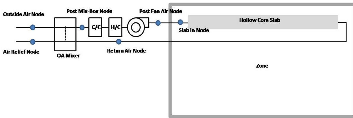
Figure 1.160: Ventilated Slab model - basic system
