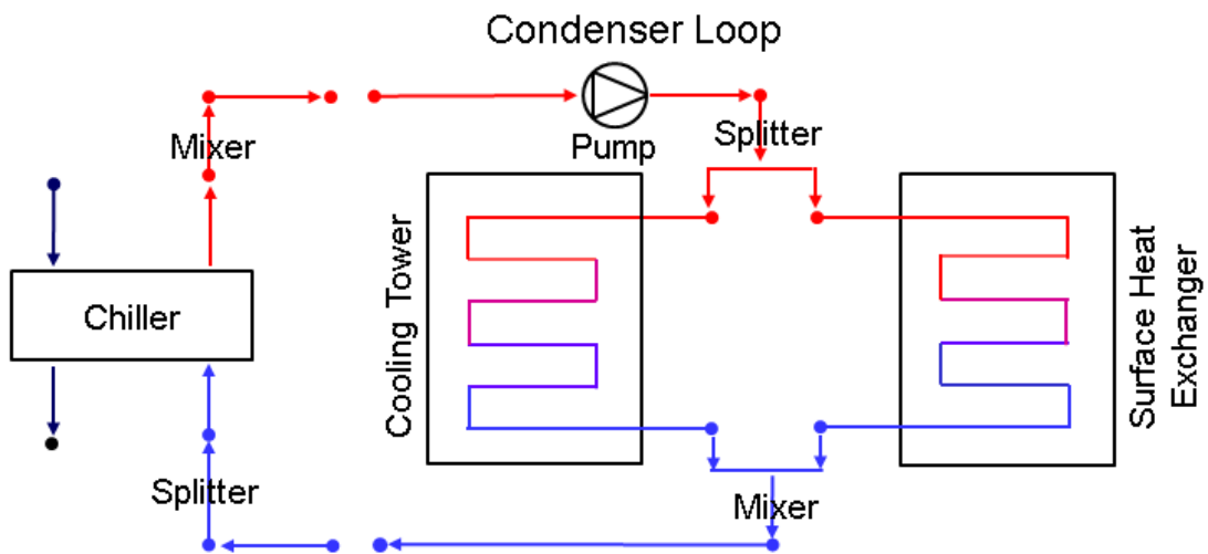
Figure 1.108: Surface Ground Heat Exchanger with other heat exchangers on condenser loop
