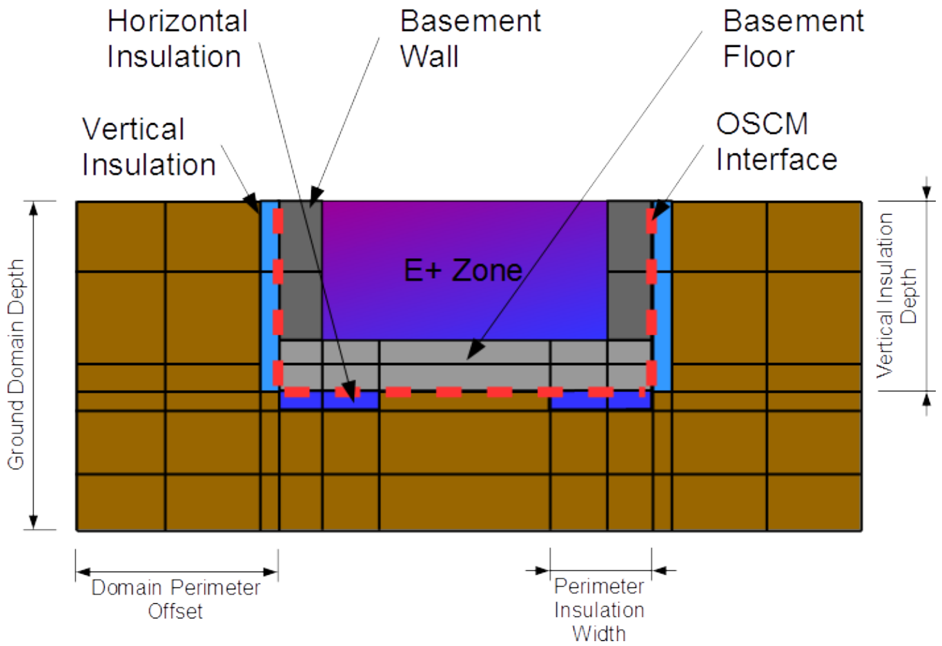
Figure 1.9: Basement Configuration
