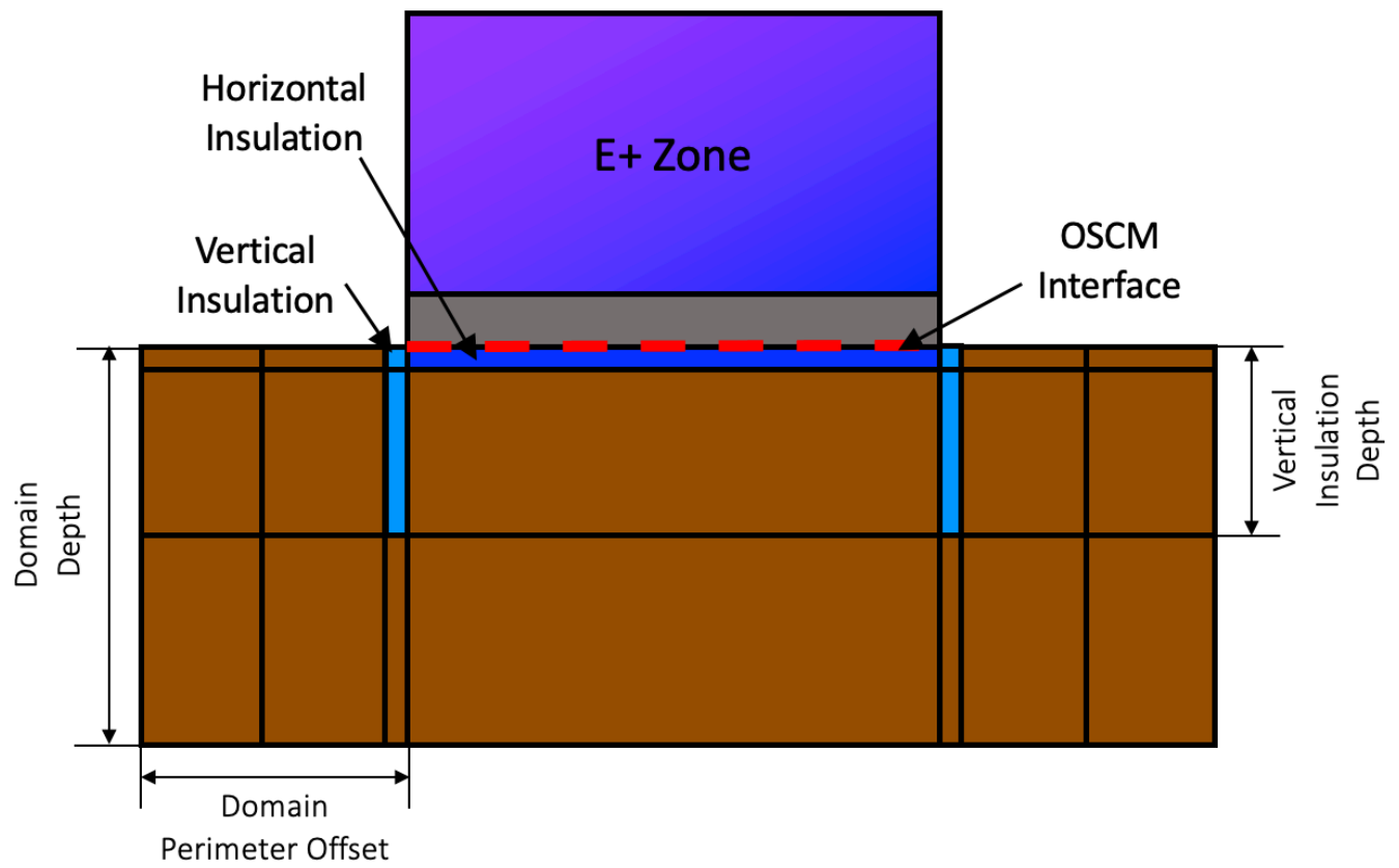
Figure 1.8: On-grade configuration
