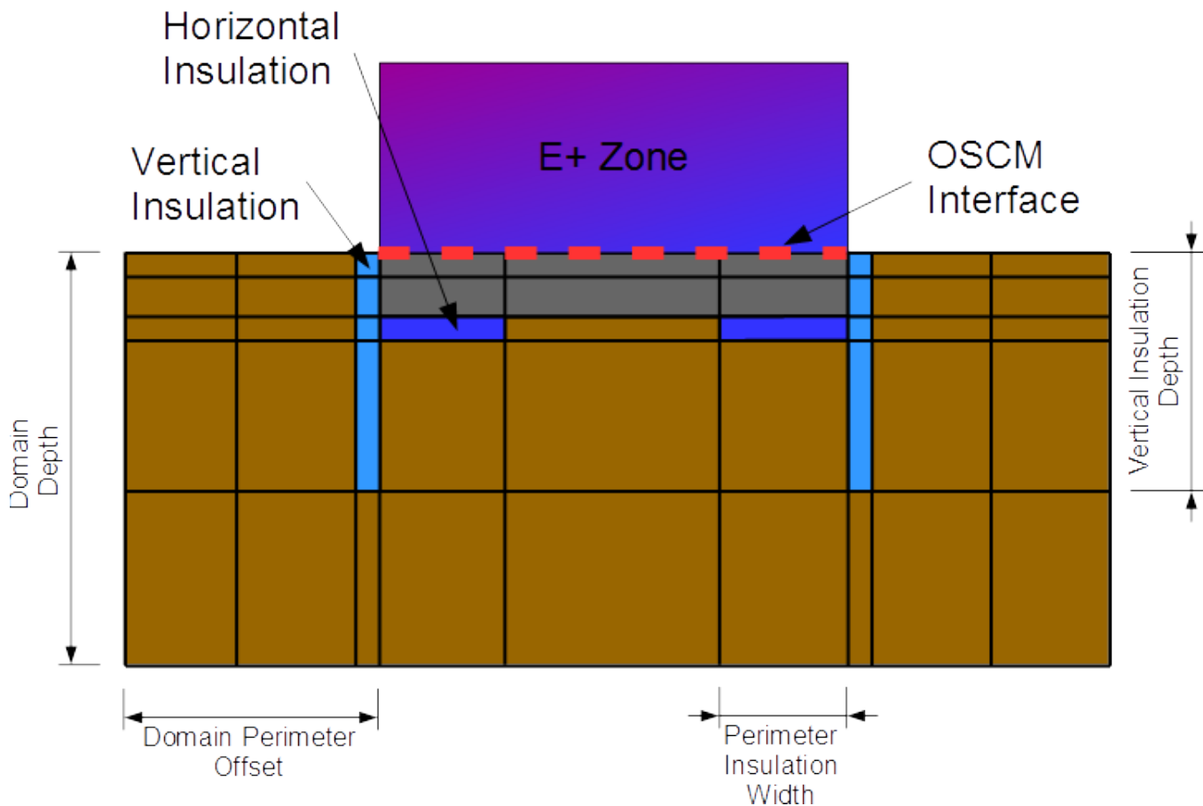
Figure 1.7: In-grade configuration.
