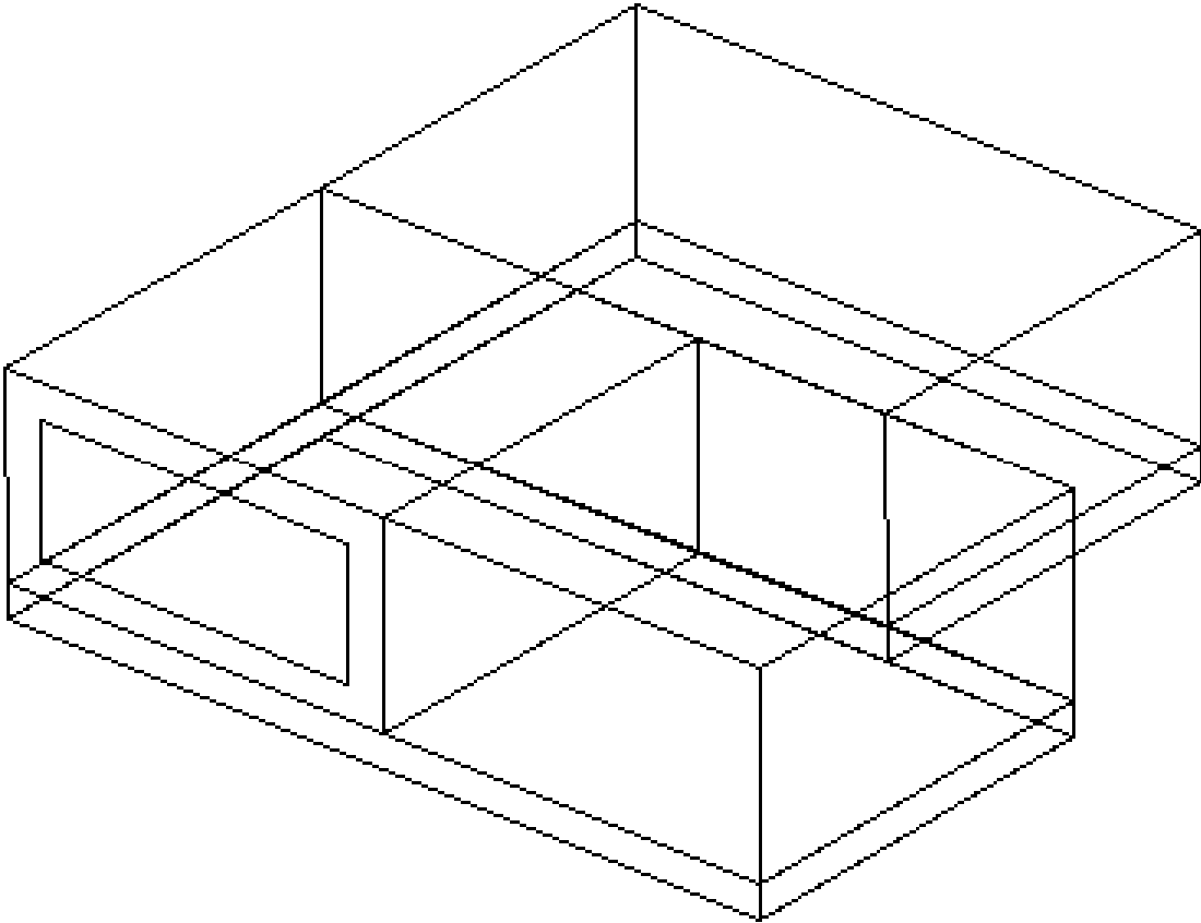
Figure 1.163: Illustration of AirLoopHVAC:SupplyPlenum
