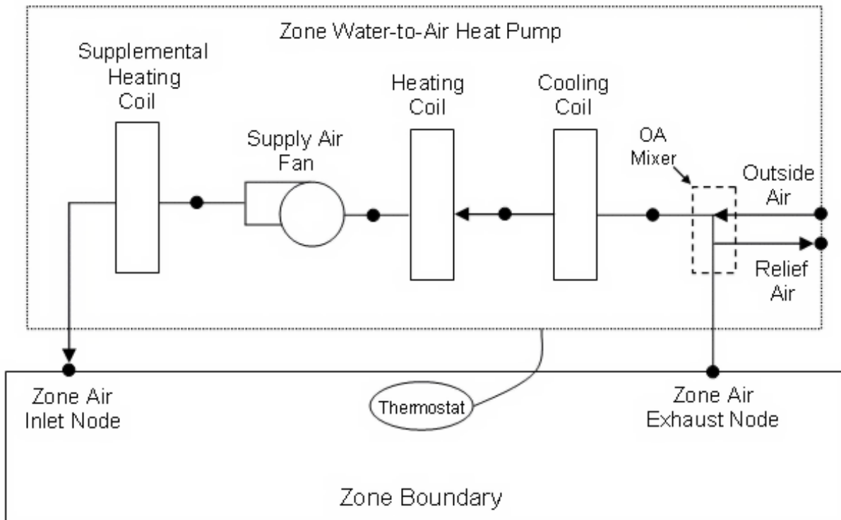
Figure 1.137: Zone Water to Air Heat Pump Schematic for a DrawThrough Configuration with Ground Heat Exchanger
