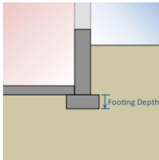
Figure 1.58: Placement of footing
