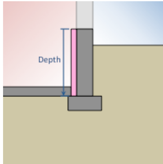
Figure 1.53: Placement of interior vertical insulation
