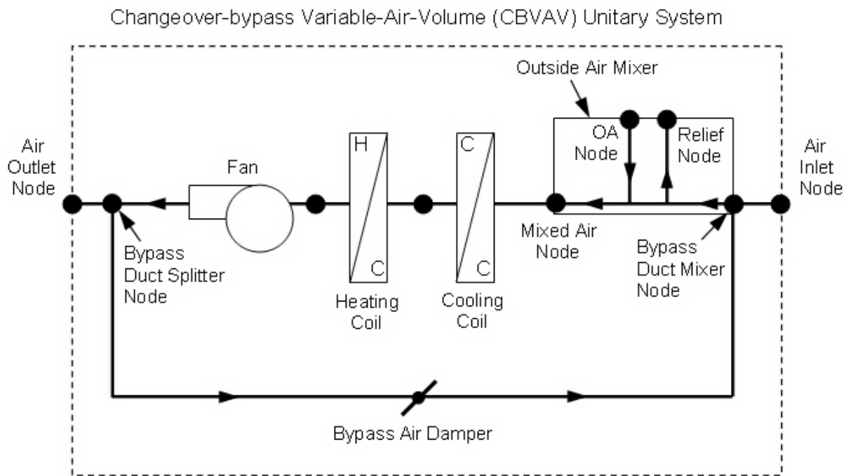
Figure 1.154: Schematic of a CBVAV unitary system (draw through fan placement)
