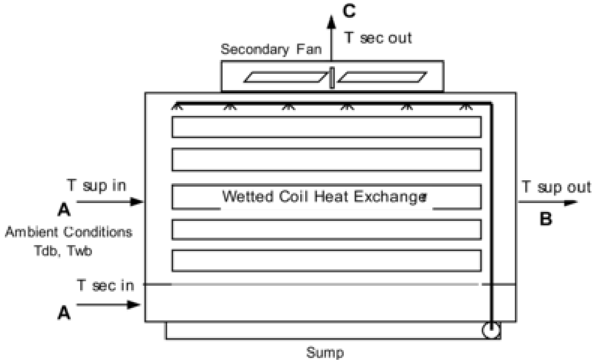
Figure 1.195: Evaporative Cooler Indirect Wet Coil
