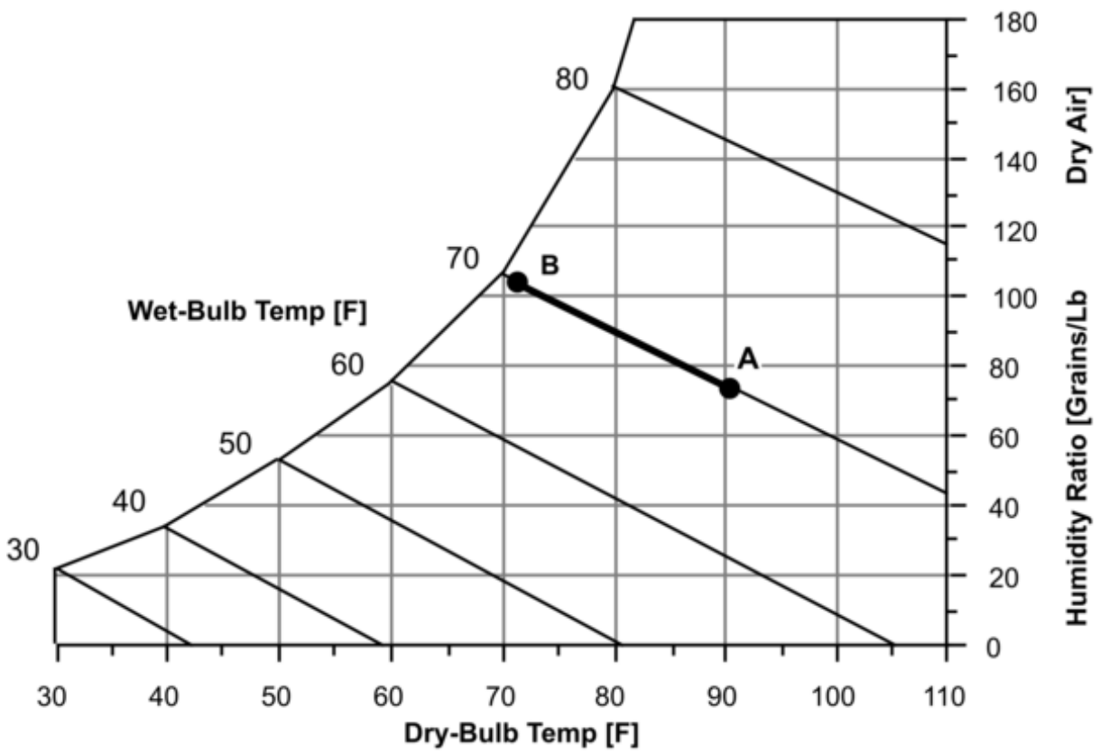
Figure 1.192: Psychrometric Chart – Constant Enthalpy
