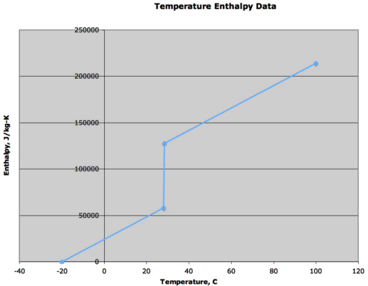
Figure 1.11: Temp-Enth Example
