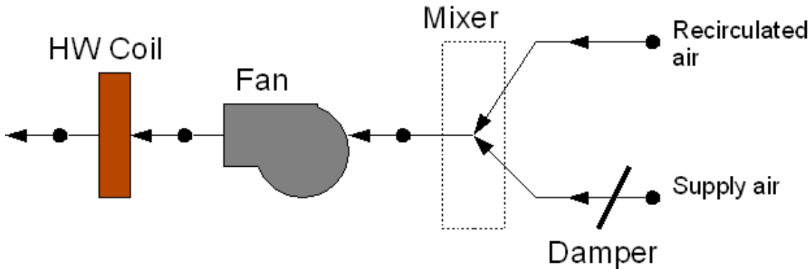
Figure 1.130: Series PIU Terminal Unit
