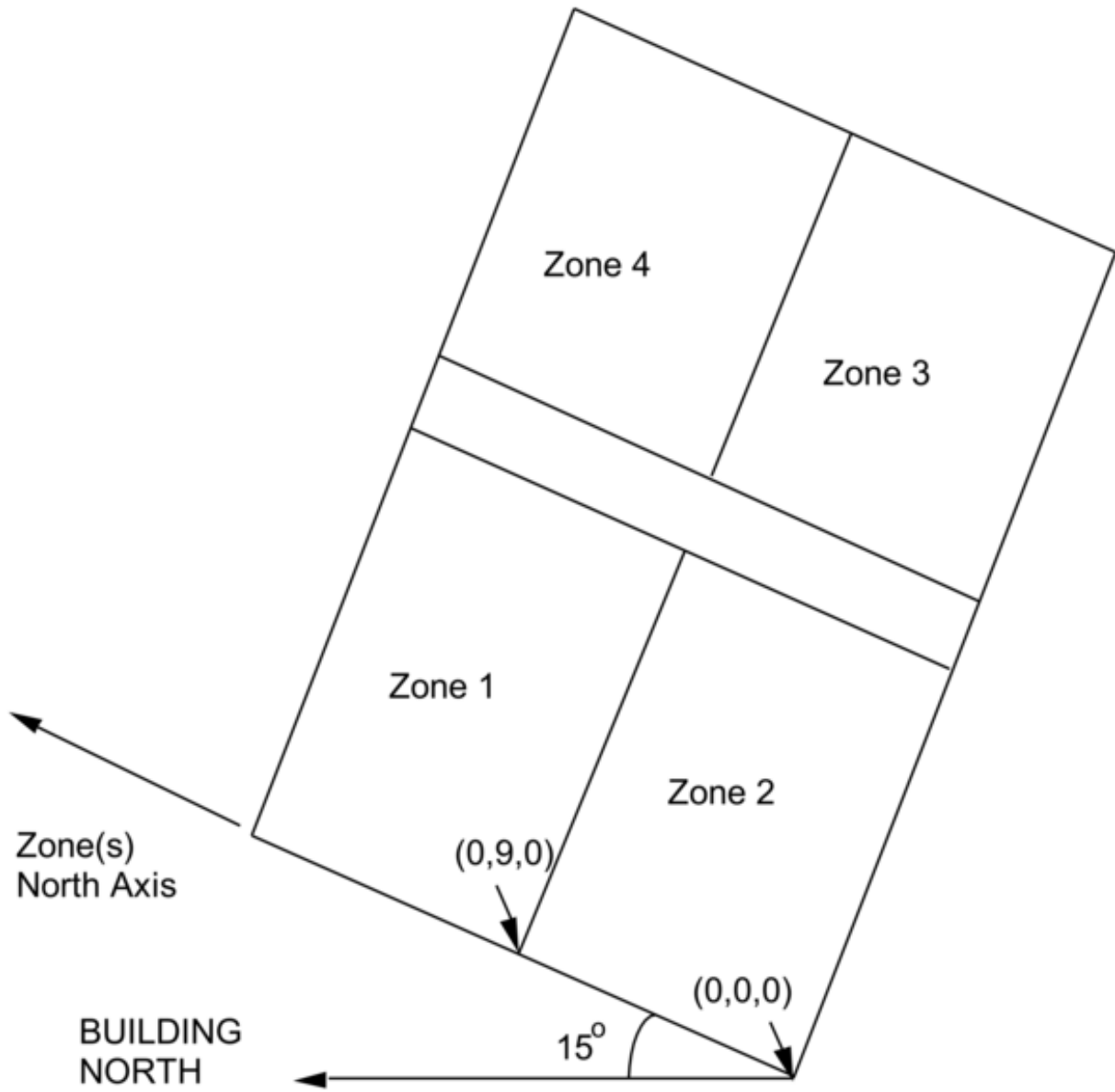
Figure 1.29: Illustration of Zone North Axis and Origins
