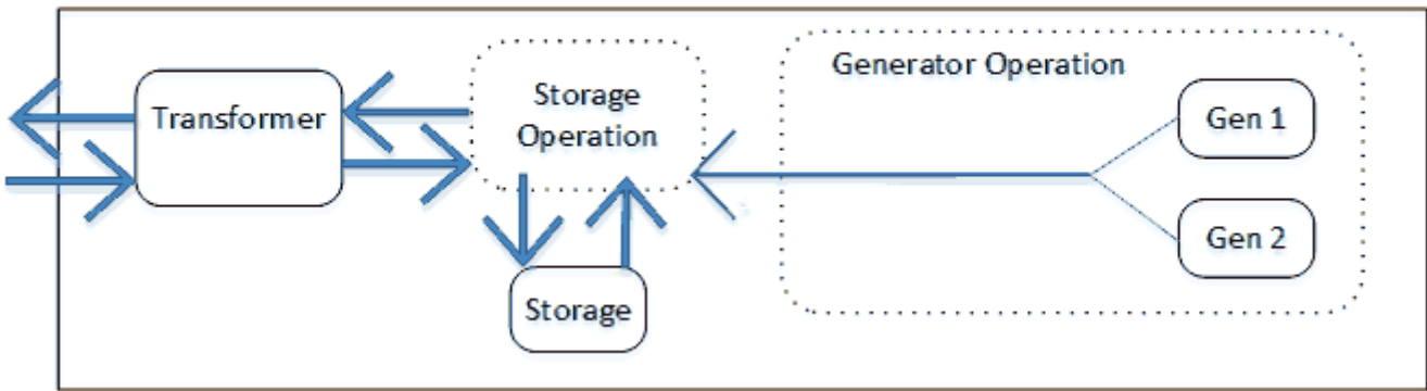
Figure 1.201: LoadCenterBusType
