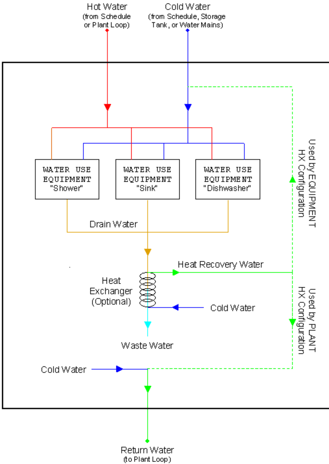
Figure 1.206: Diagram of internal connections for WaterUse:Connections
