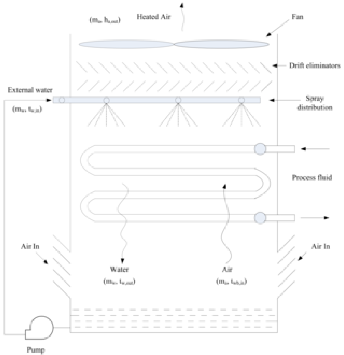
Figure 1.101: Schematic diagram for evaporative fluid cooler
