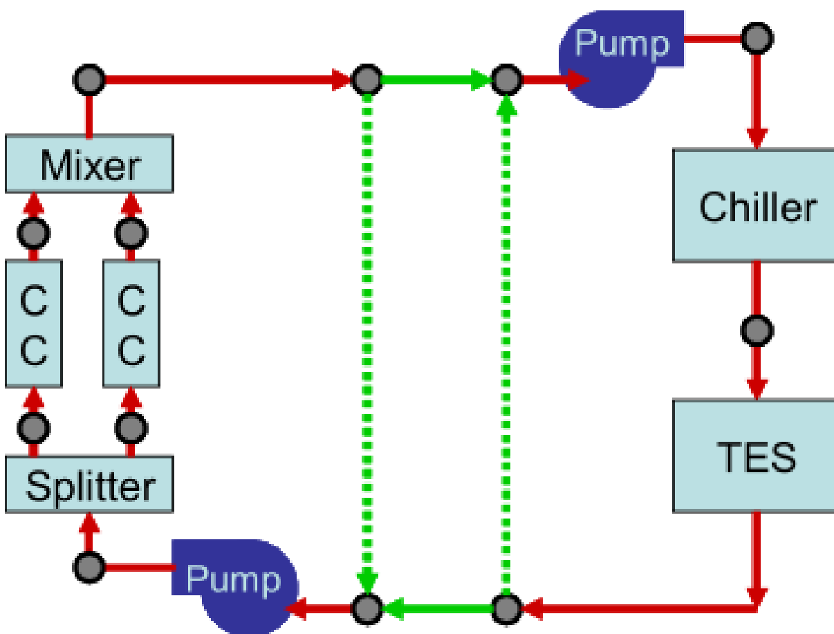
Figure 9.9: Schematic of a Two-Way Common Pipe used in Primary-Secondary System.
