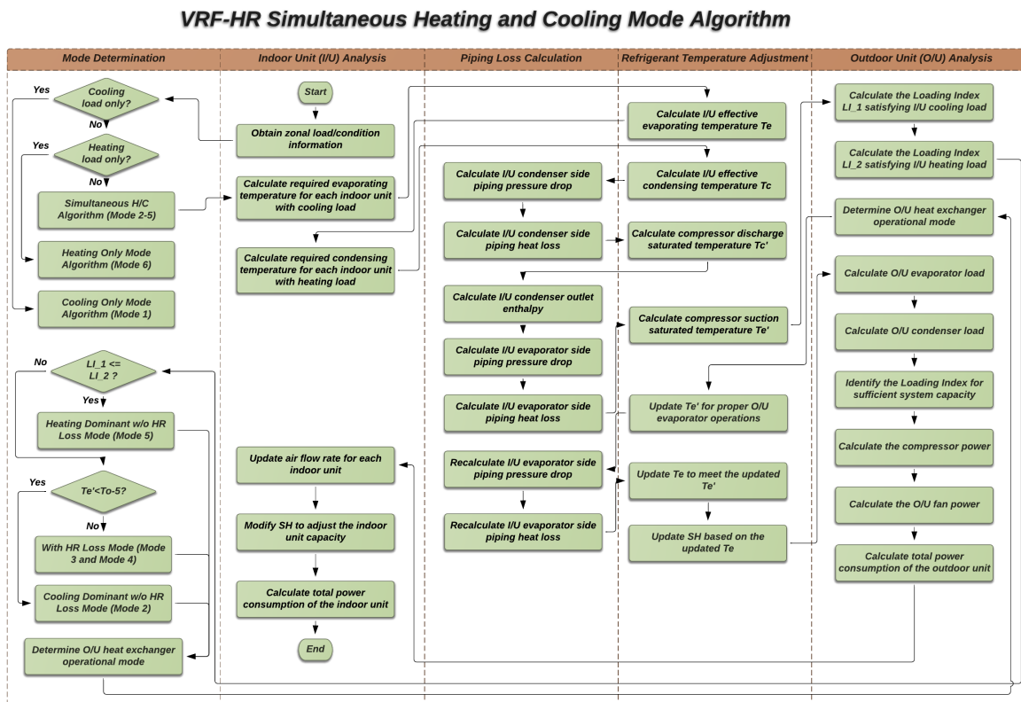
Figure 16.70: Schematic chart of the new VRF-HR algorithm: Simultaneous Heating and Cooling Mode
