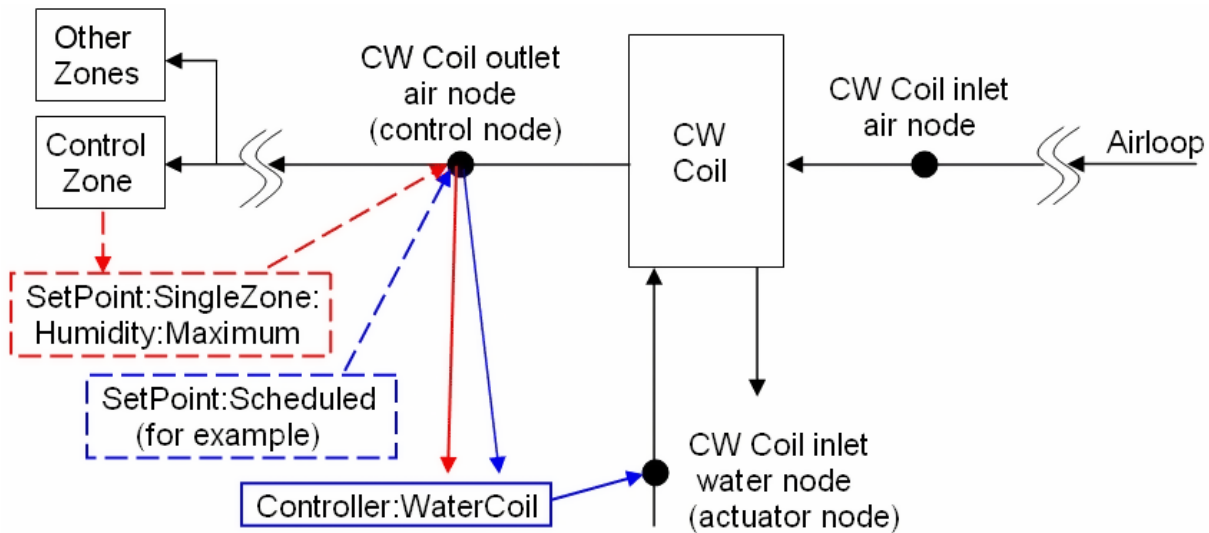
Figure 15.31: Two Setpoint managers used in Controller:WaterCoil
