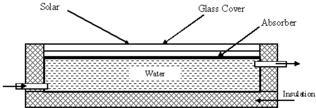
Figure 18.35: Schematic diagram of rectangular Integrated Collector Storage unit
