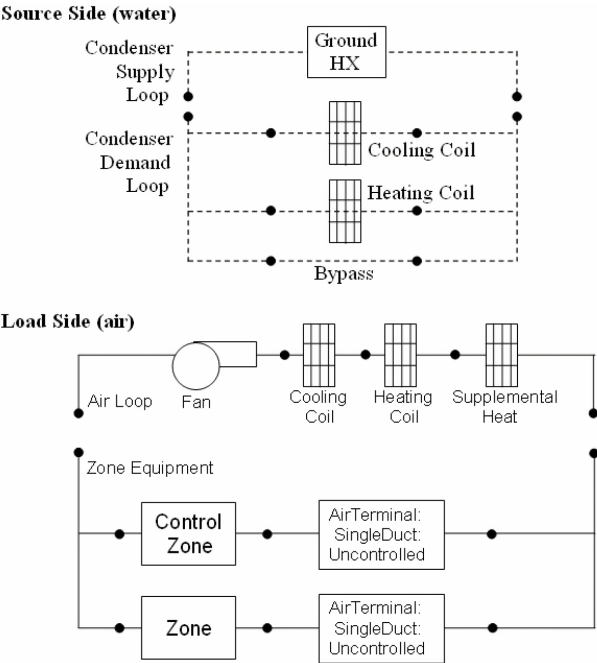
Figure 16.43: Source Side and Load Side Configuration of a BlowThru Water-To-Air Heat Pump
