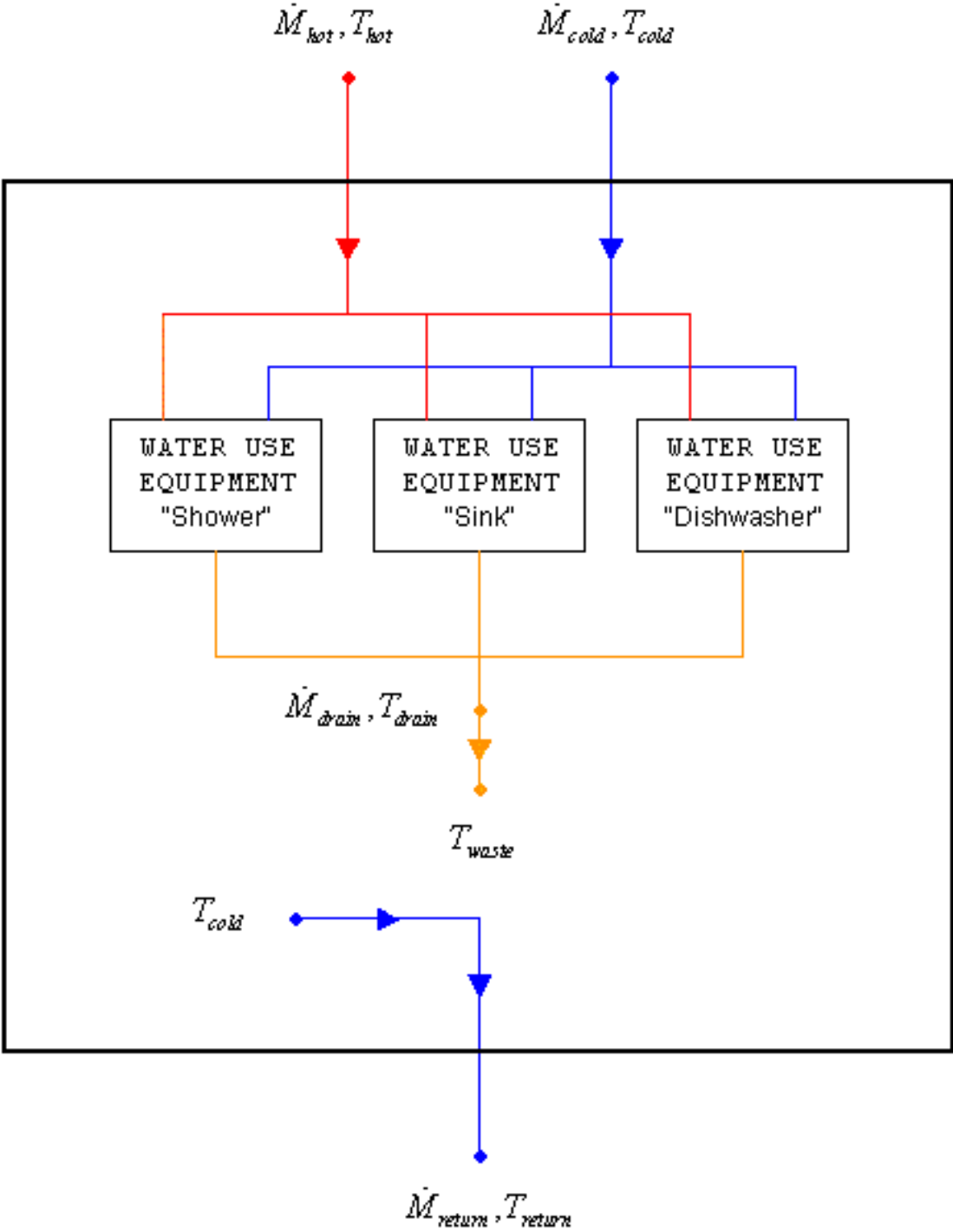
Figure 19.18: Water Use Connections Subsystem
