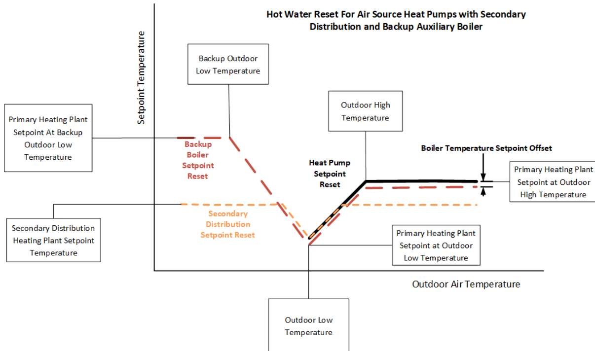
Figure 9.6: Hot Water Temperature Setpoint Vs Outdoor Air Temperature
