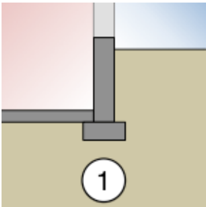
Figure 3.32: Group 1 Kiva context
