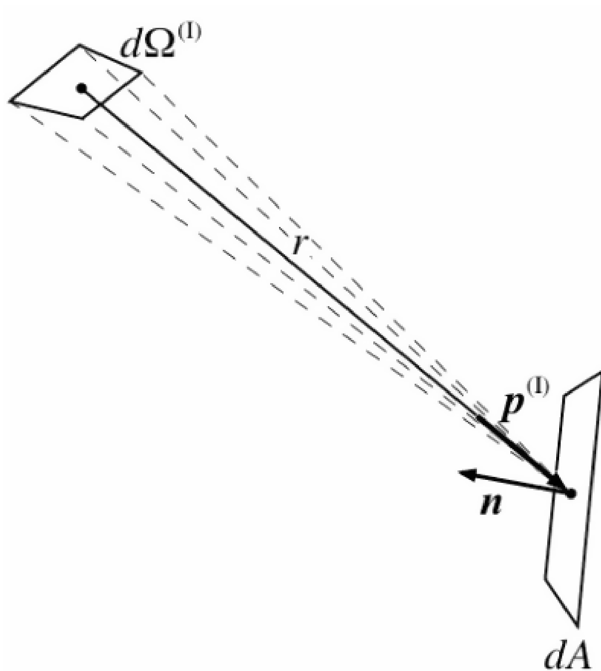
Figure 7.34: Irradiance geometry
