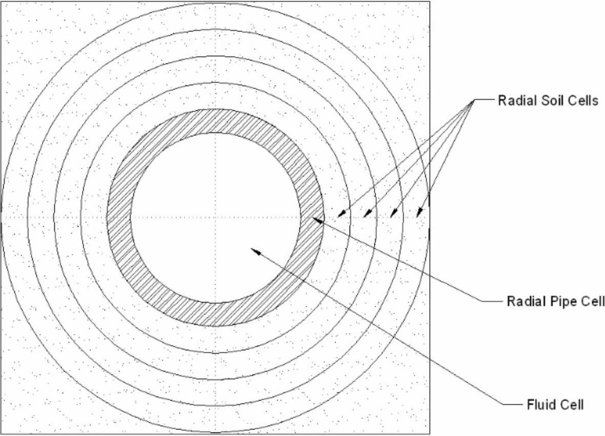
Figure 17.6: Close-up view of example radial cell
