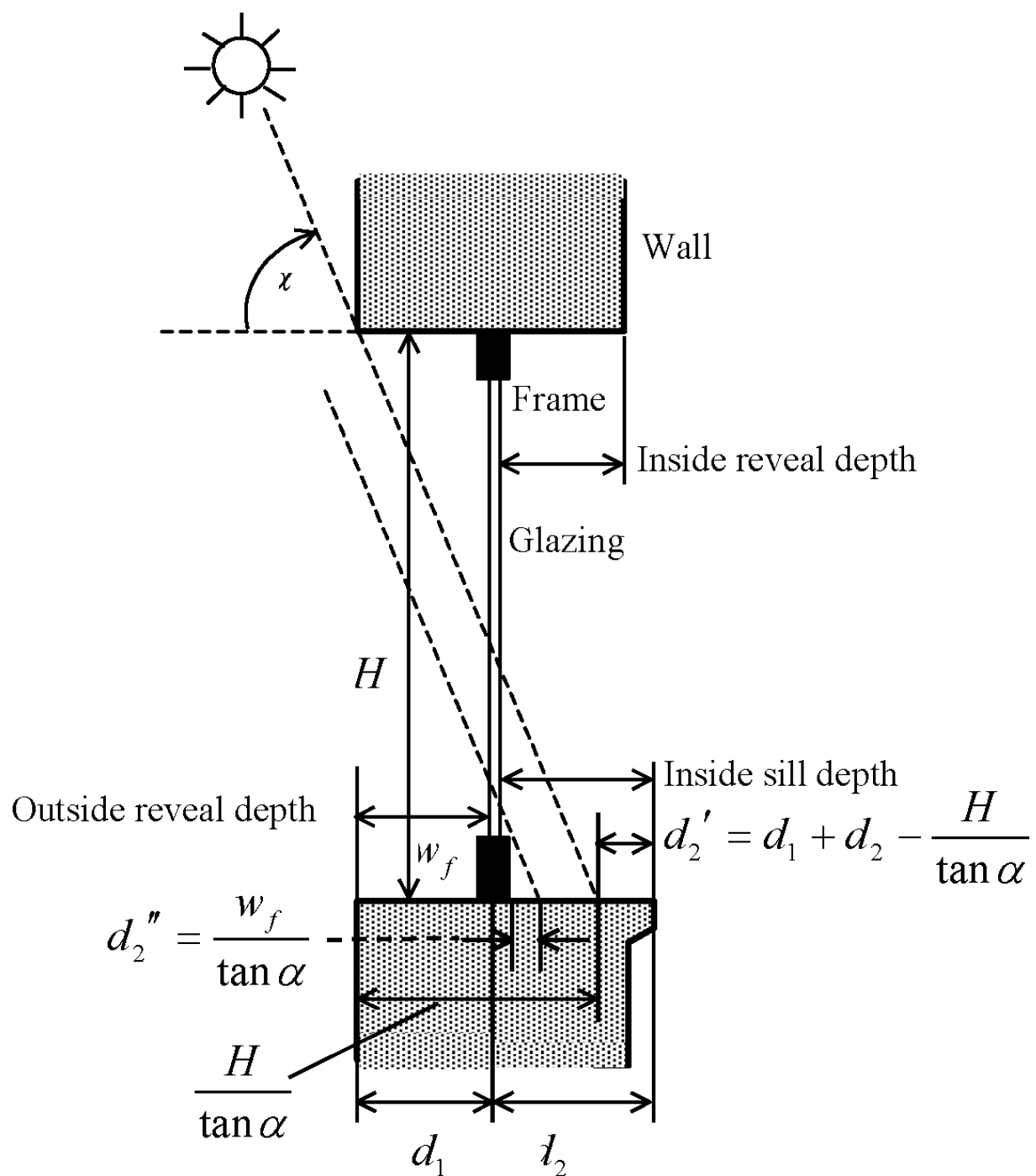
Figure 7.45: Vertical section through a vertical window with outside and inside reveal showing calculation of the shadows cast by the top reveal onto the inside sill and by the frame onto the inside sill.
