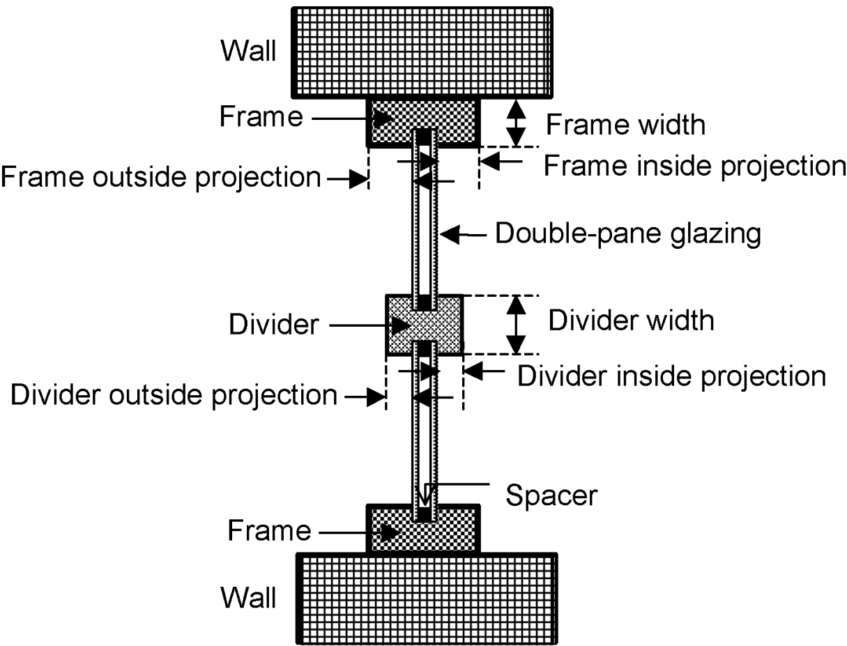
Figure 7.41: Cross section through a window showing frame and divider (exaggerated horizontally).
