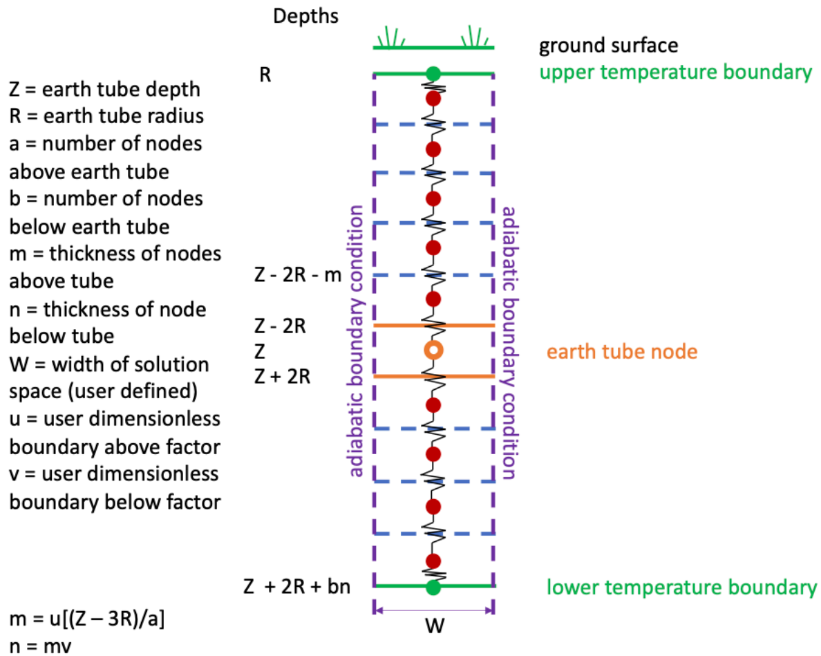
Figure 19.35: Earth Tube Vertical Model Solution Space
