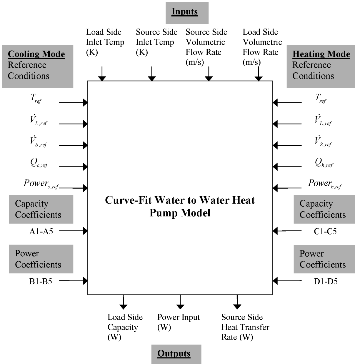
Figure 16.47: Information Flow Chart for Water-To-Water Heat Pump Equation Fit (Tang 2005)
