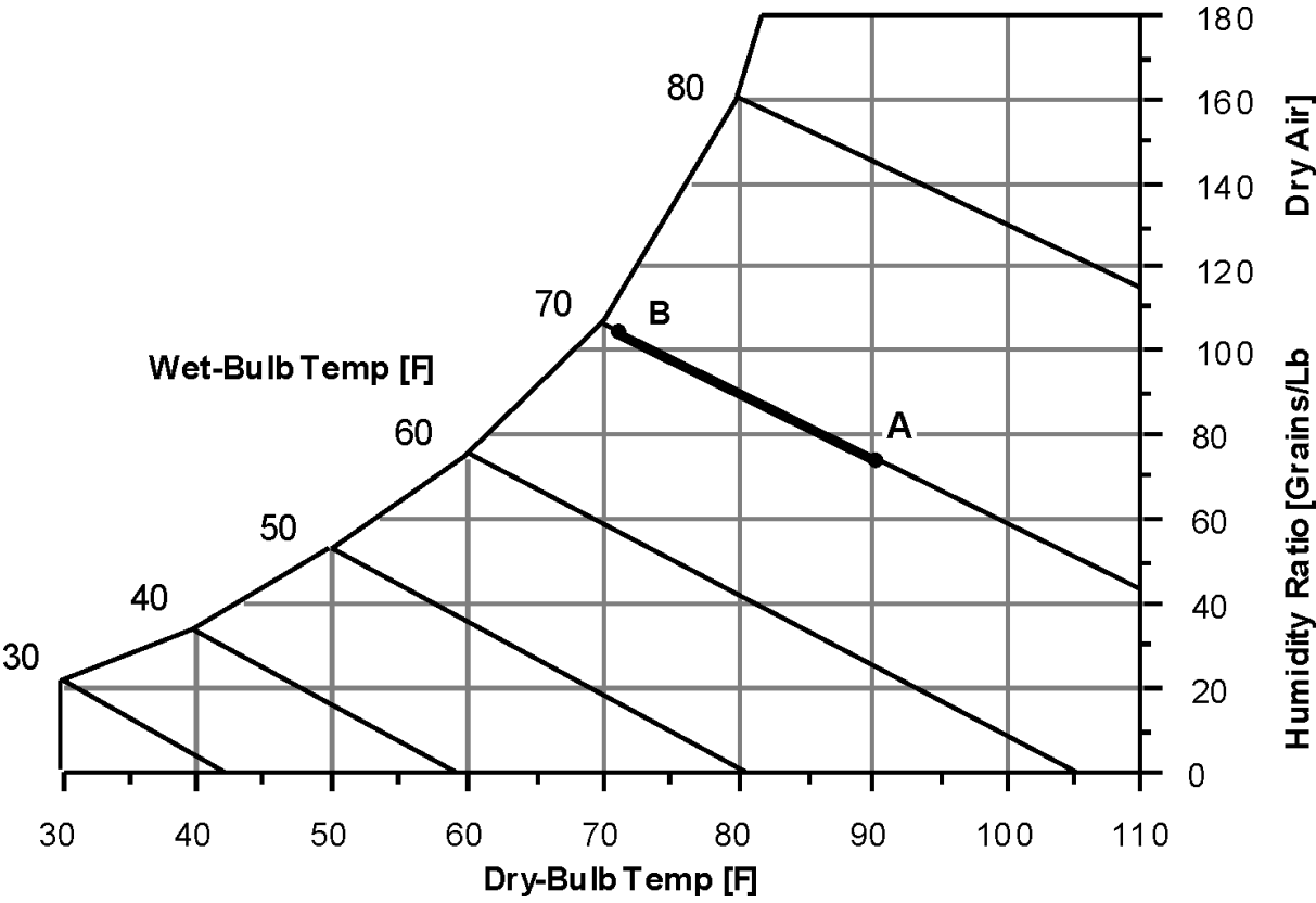
Figure 16.5: Psychrometric Chart – Constant Enthalpy
