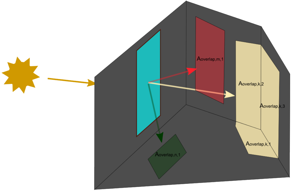
Figure 7.8: Complex Fenestration System Light Patches
