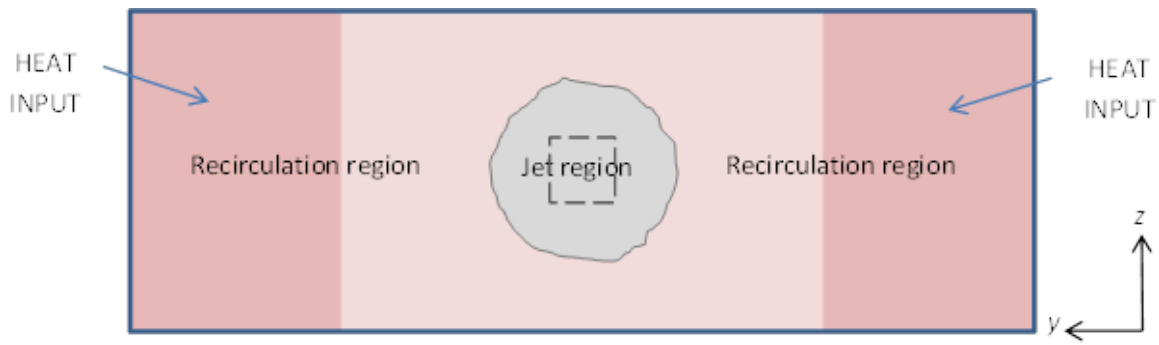
Figure 13.21: Jet and recirculation regions in typical vertical cross-section through room (y-z plane). Jet boundary occurs where jet velocity has fallen to 50% of centerline maximum. Remainder of cross-section is treated as recirculation. Volumetric heat sources are
