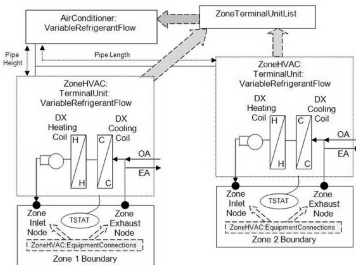
Figure 19.28: Zone Terminal Unit Schematic
