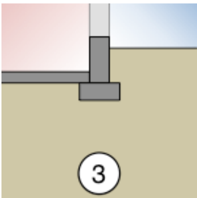
Figure 3.34: Group 3 Kiva context
