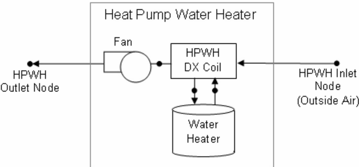
Figure 19.14: Schematic of a Heat Pump Water Heater with Inlet Air from Outdoors
