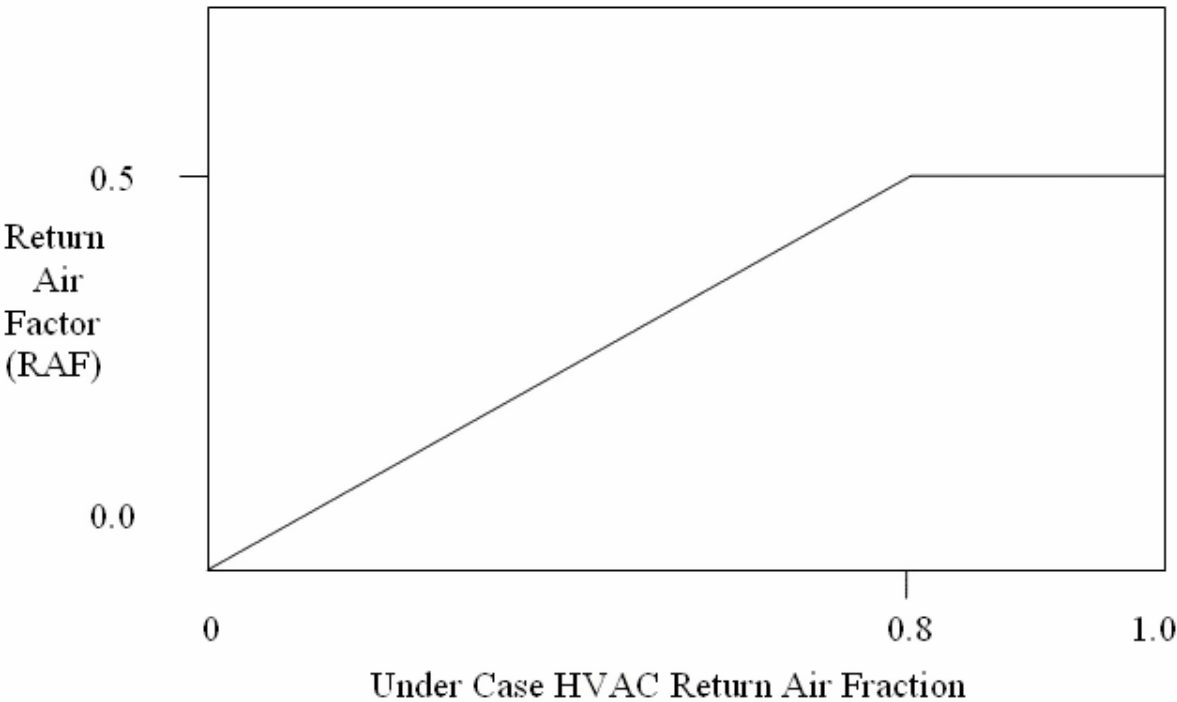
Figure 18.16: Return Air Factor Versus Under Case HVAC Return Air Fraction
