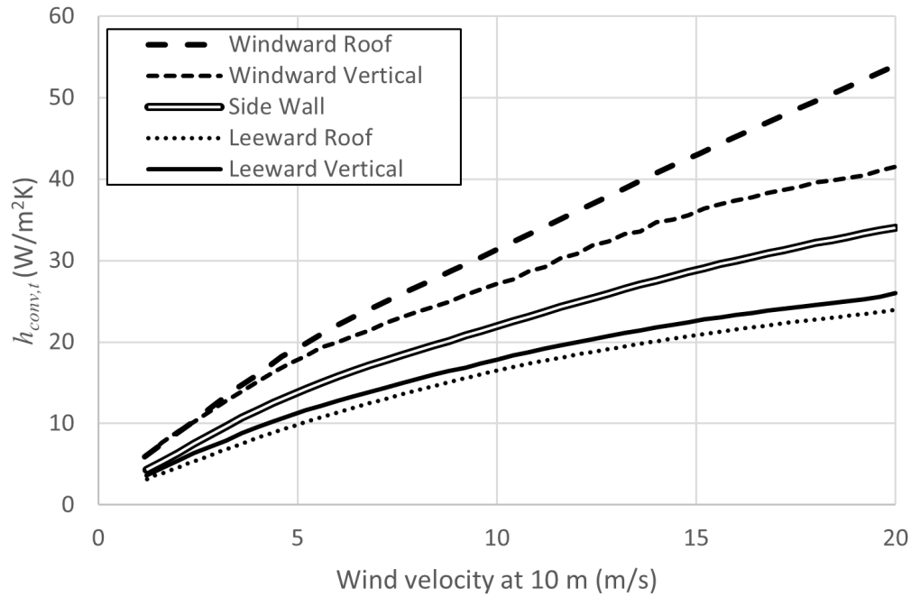
Figure 18.42: Results by Gorman et al. (2019) for external heat transfer coefficients on buildings. Reproduced from Gorman et al., 2019.
