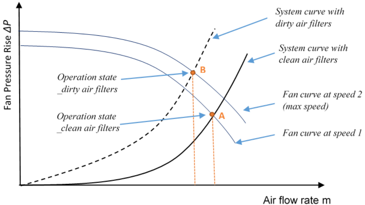
Figure 11.2: Effect of dirty air filter on variable speed fan operation – flow rate reduced
