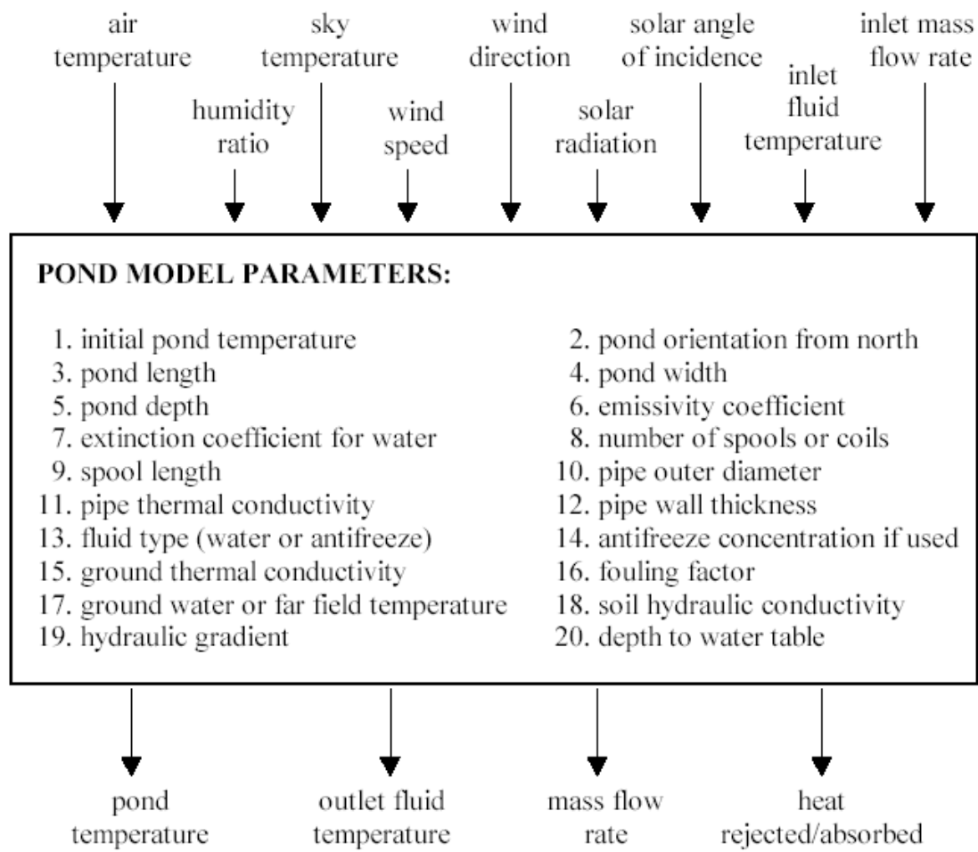
Figure 16.80: Pond Model Component Configuration (Chiasson 1999)
