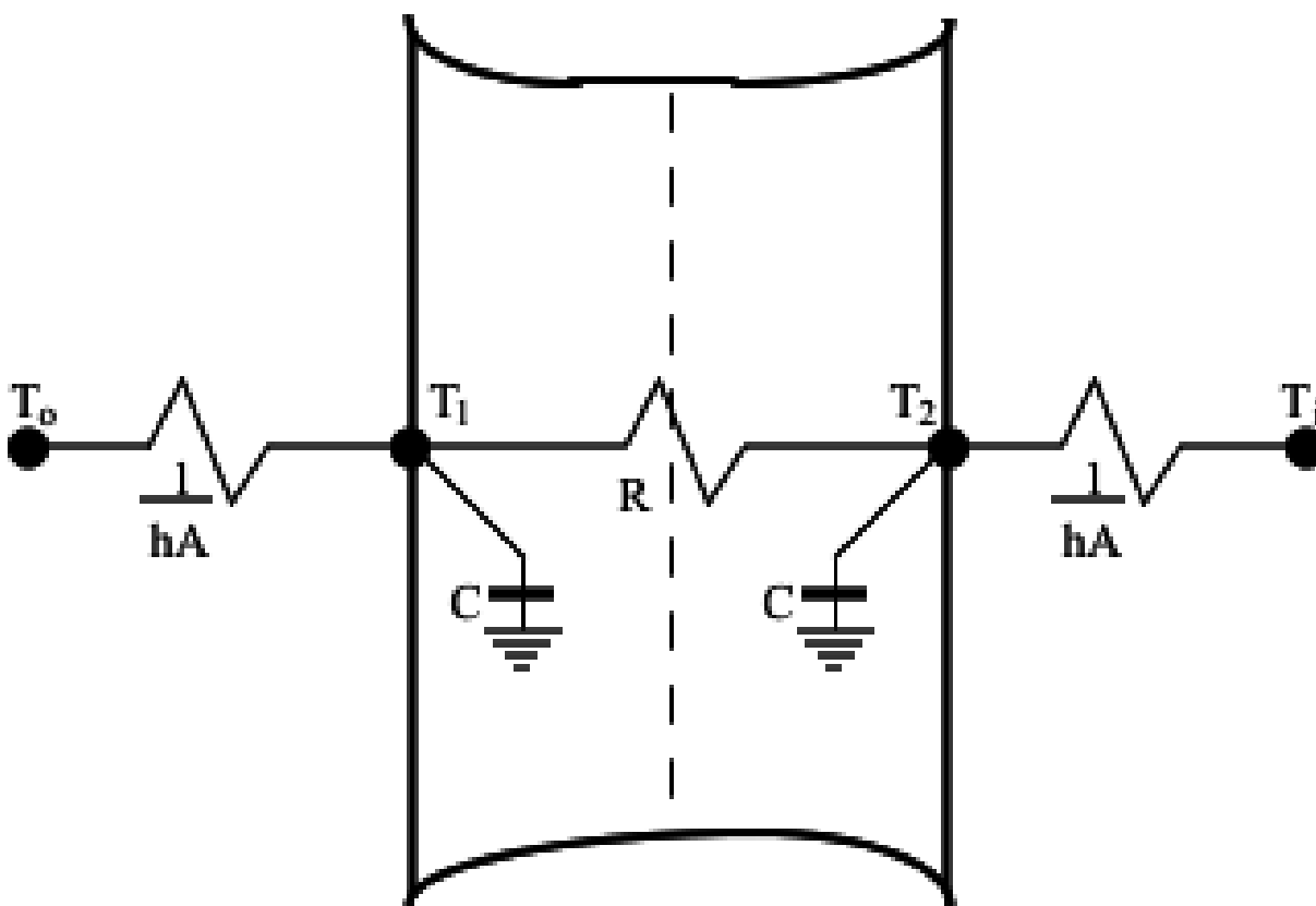
Figure 3.1: Two Node State Space Example.
