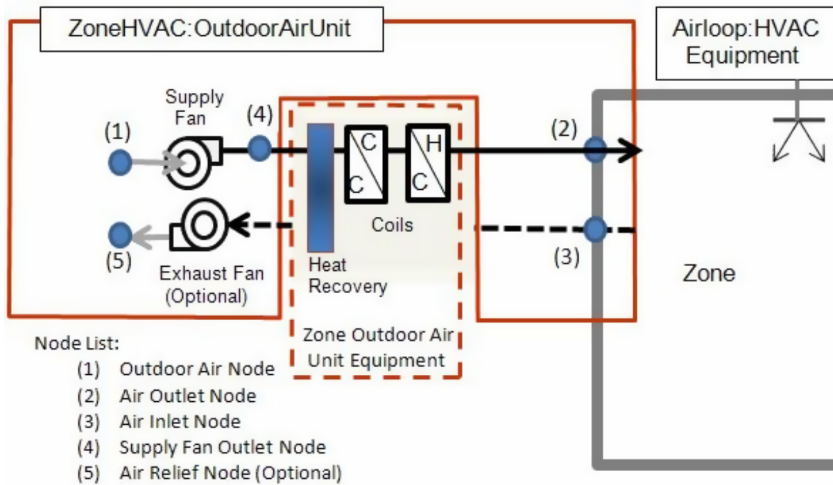
Figure 19.37: Zone Outdoor Air Unit Schematic
