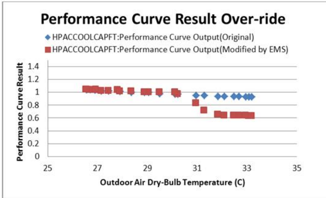
Figure 8.1: Results of Performance Curve Override
