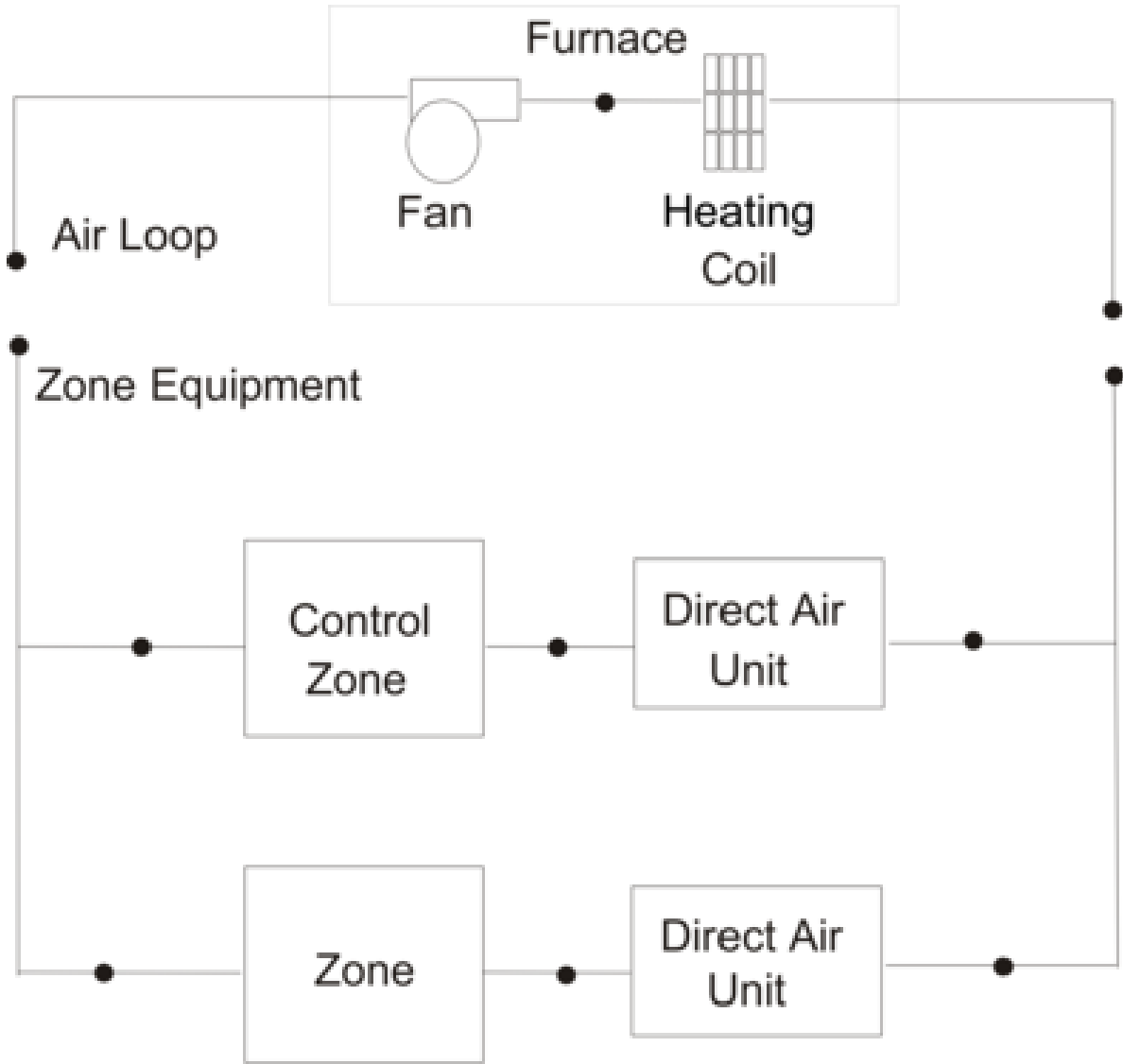
Figure 1.158: Schematic of Blow Through Furnace Model
