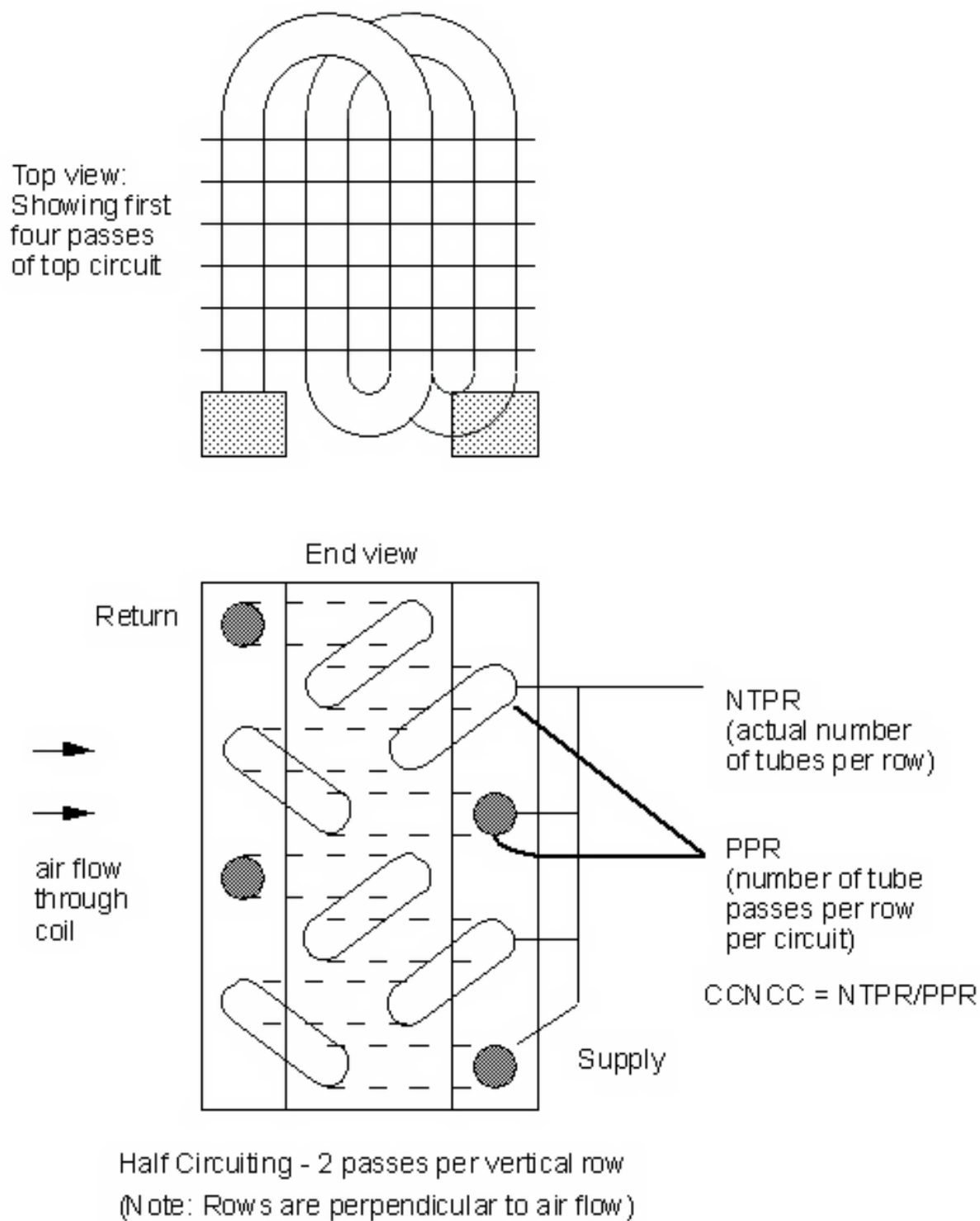
Figure 1.177: Number of Coolant Circuits (CCNCC)
