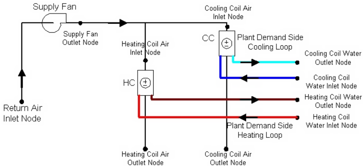
Figure 1.175: Example Air Loop Heating &amp; Cooling Coil
