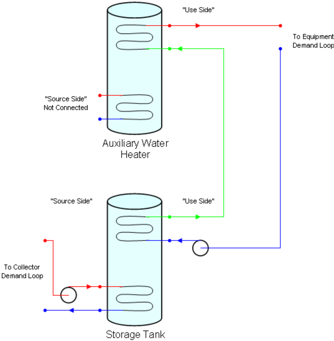
Figure 1.172: Two-Tank Solar Heating System Connection Diagram
