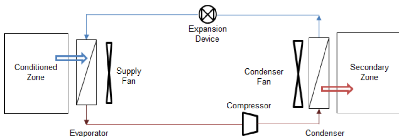
Figure 1.192: Schematic of DX System and heat pump in cooling operating mode
