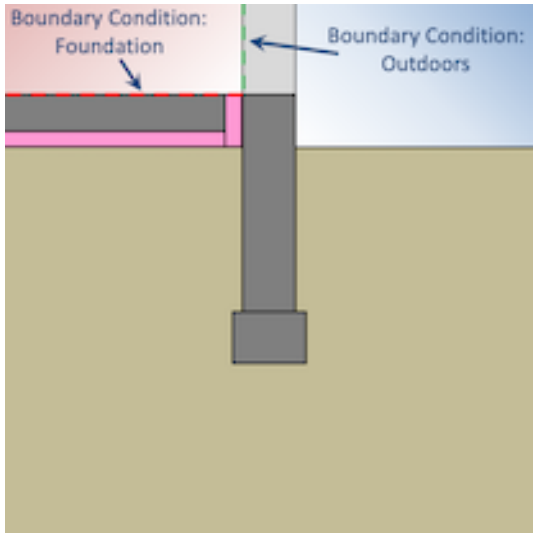
Figure 1.49: Two-dimensional interpretation of foundation surface data
