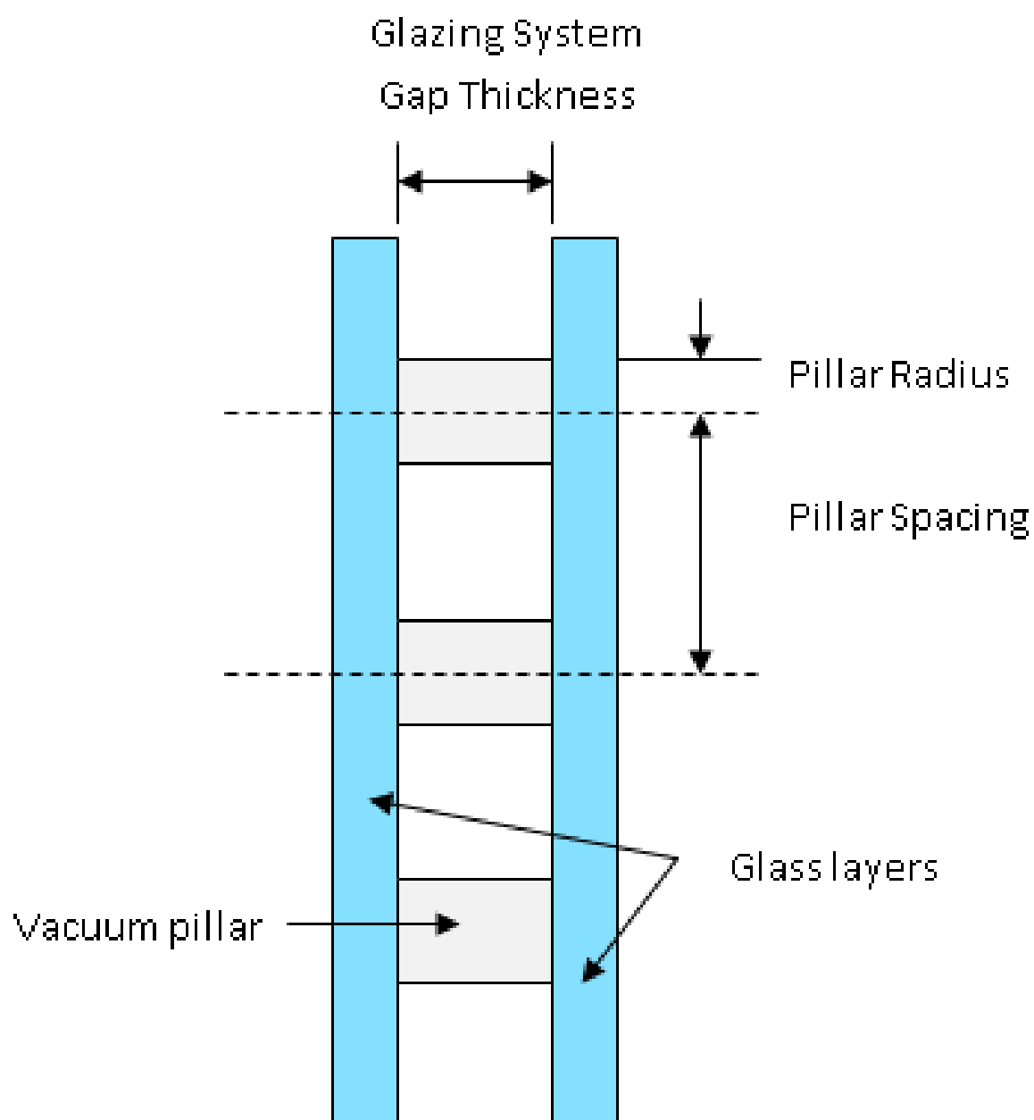
Figure 1.13: Support Pillar
