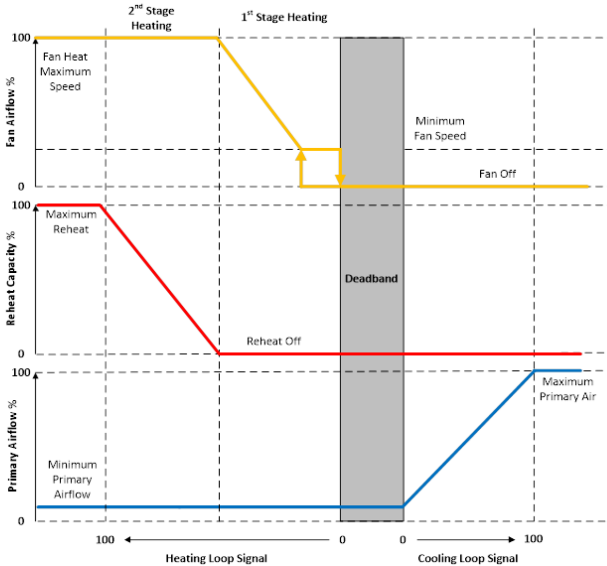
Figure 1.137: Variable Speed Fan with Staged Heat Control
