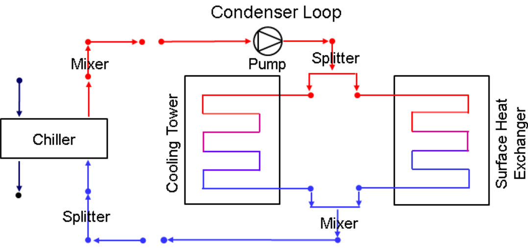
Figure 1.110: Surface Ground Heat Exchanger with other heat exchangers on condenser loop
