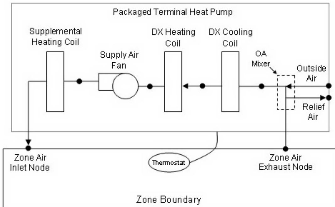
Figure 1.143: Schematic of a packaged terminal heat pump (draw through fan placement)
