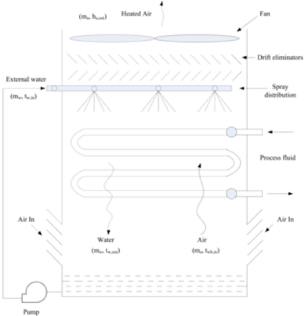
Figure 1.103: Schematic diagram for evaporative fluid cooler
