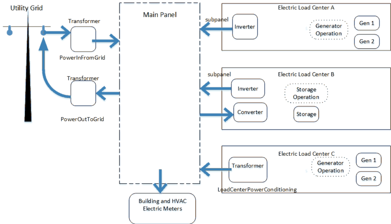
Figure 1.206: PowerServiceOverview
