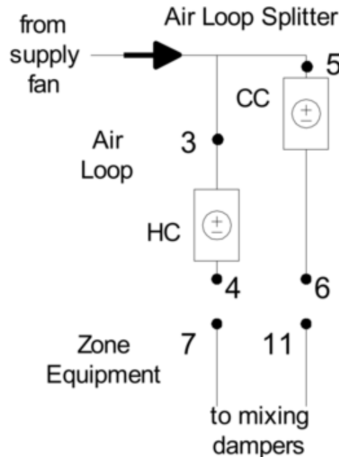
Figure 1.126: Air Loop/Zone Equipment Node Diagram
