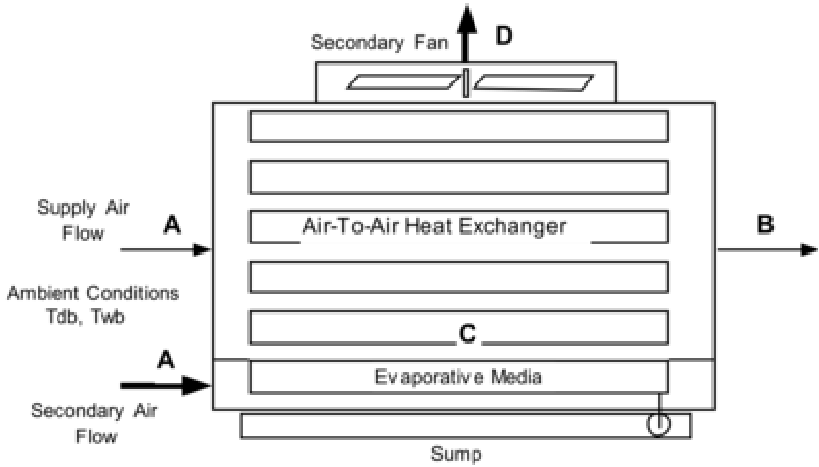
Figure 1.200: Evaporative Cooler – Indirect Dry Coil
