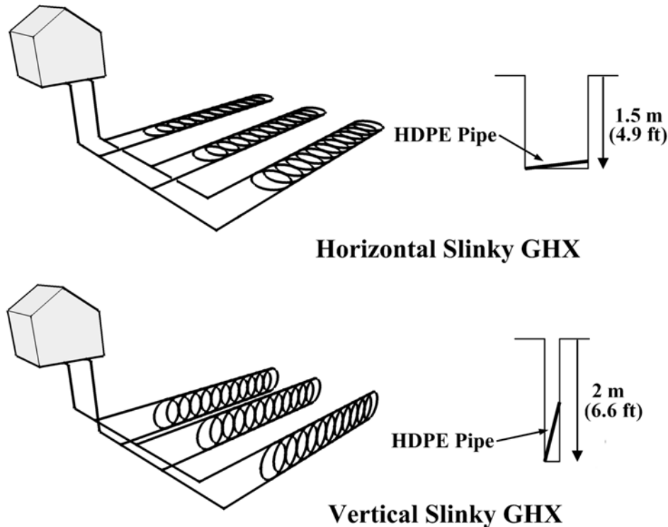
Figure 1.105: slinky heat exchanger
