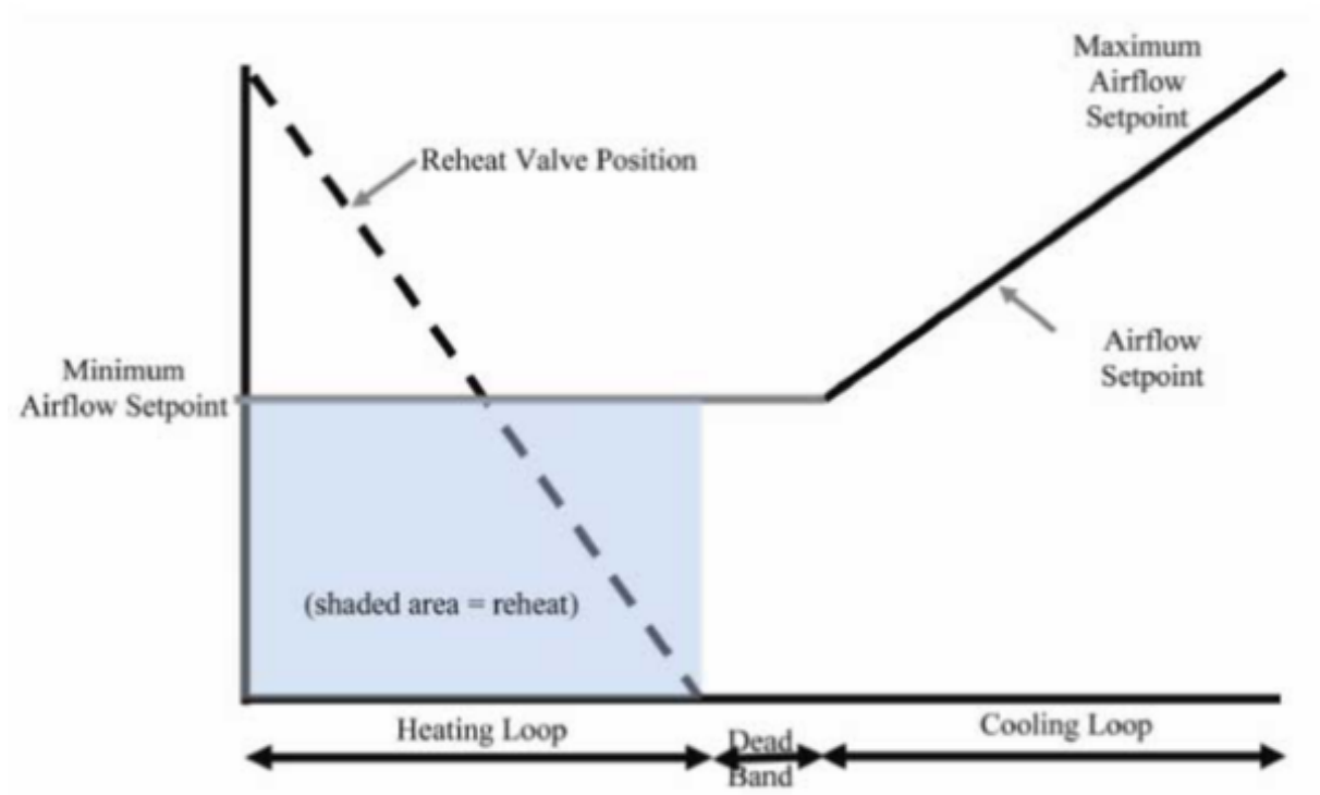
Figure 1.129: The Single Maximum Control Logic
