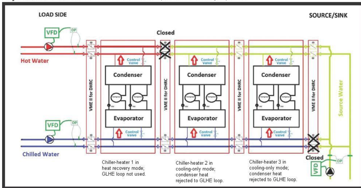
Figure 1.99: Diagram of a central heat pump system with one chiller-heater in heat recovery mode and two chiller-heaters in cooling-only mode
