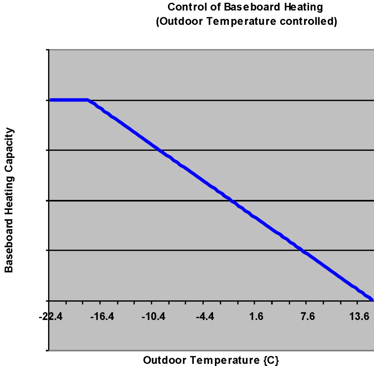
Figure 17.2: Control of Outdoor Temperature Controlled Baseboard Heat
