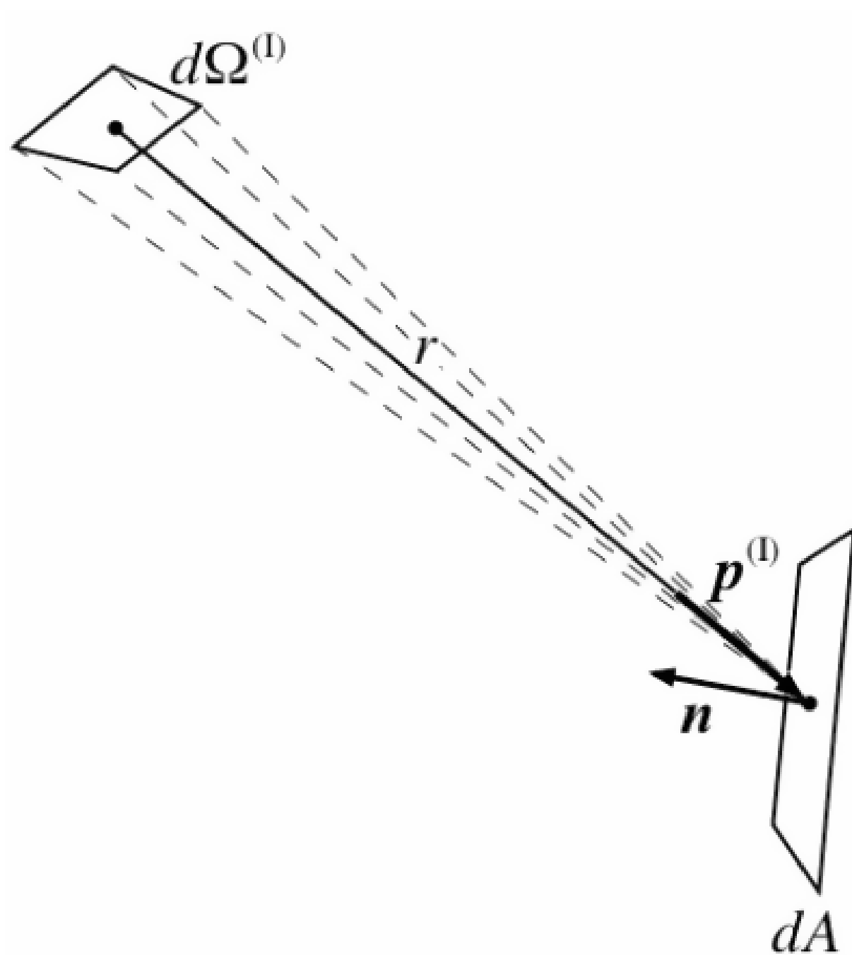
Figure 7.34: Irradiance geometry
