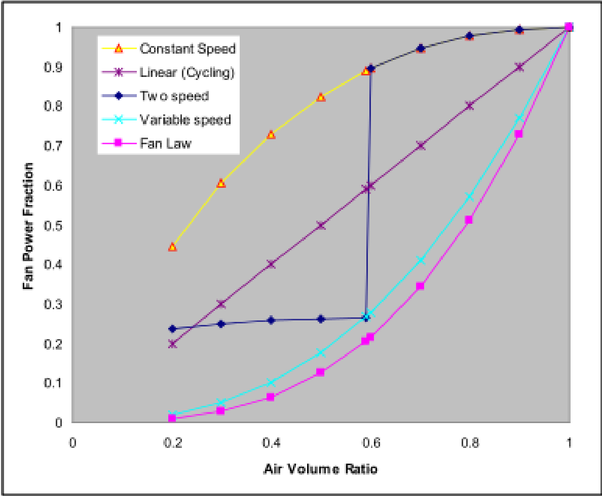
Figure 18.20: Condenser fan power curve options
