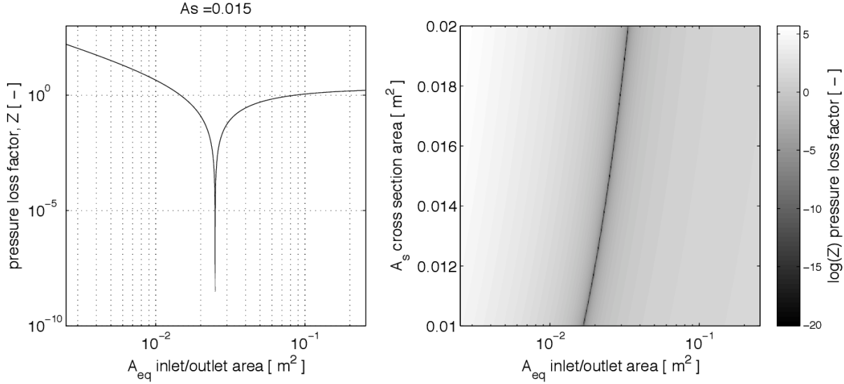
Figure 7.51: Pressure loss factor, Z , as a function of A_{eq} at A_s = 0.015 \text{ m}^2 ; and (b) surface plot of Z as a function of A_s and A_{eq} for a 1m x 1m window. The minimum follows the predicted ratio of 5/3 between A_{eq} and A_s .
