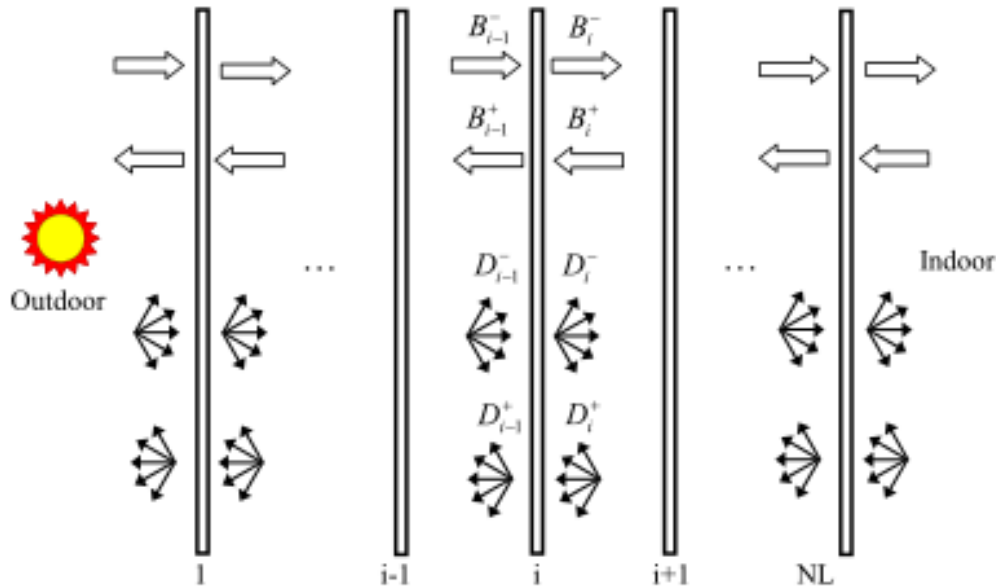
Figure 7.61: Solar analysis of the multi-layer glazing/shading system showing beam and diffuse fluxes (ASHRAE 1311-RP)
