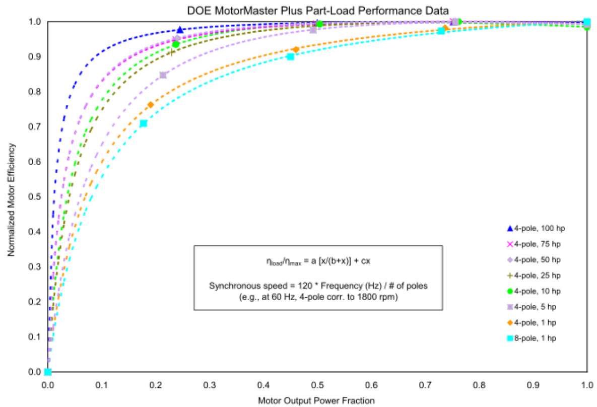
Figure 16.23: Motor Normalized Efficiency vs. Motor Load Fraction
