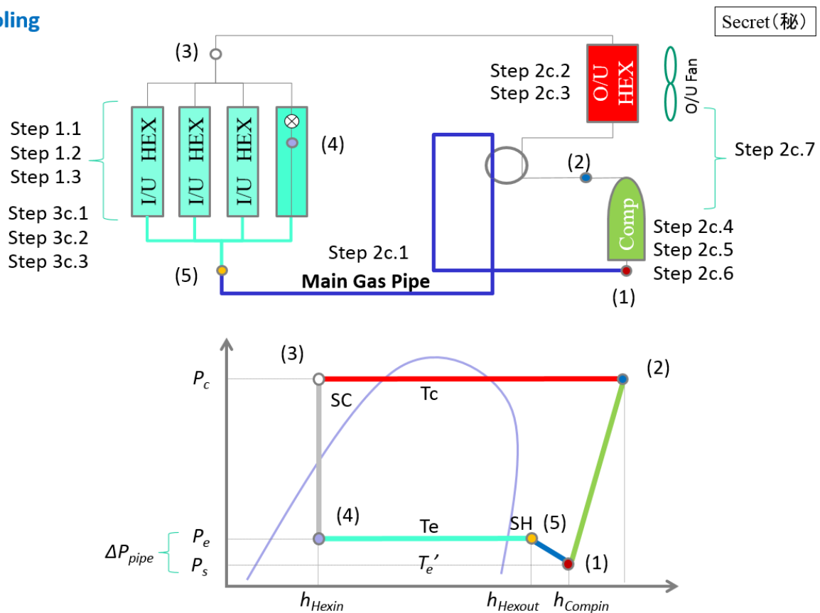
Figure 16.62: Schematic Pressure-Enthalpy Diagram for VRF Operation – Cooling Mode
