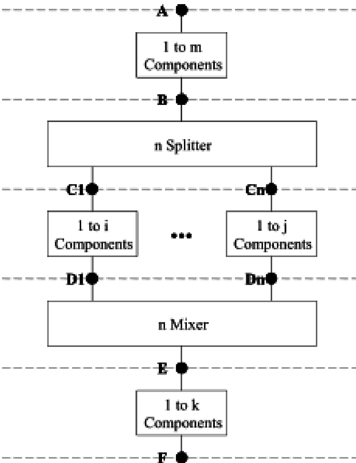
Figure 9.2: Branch Layout for Individual Plant Half-Loops
