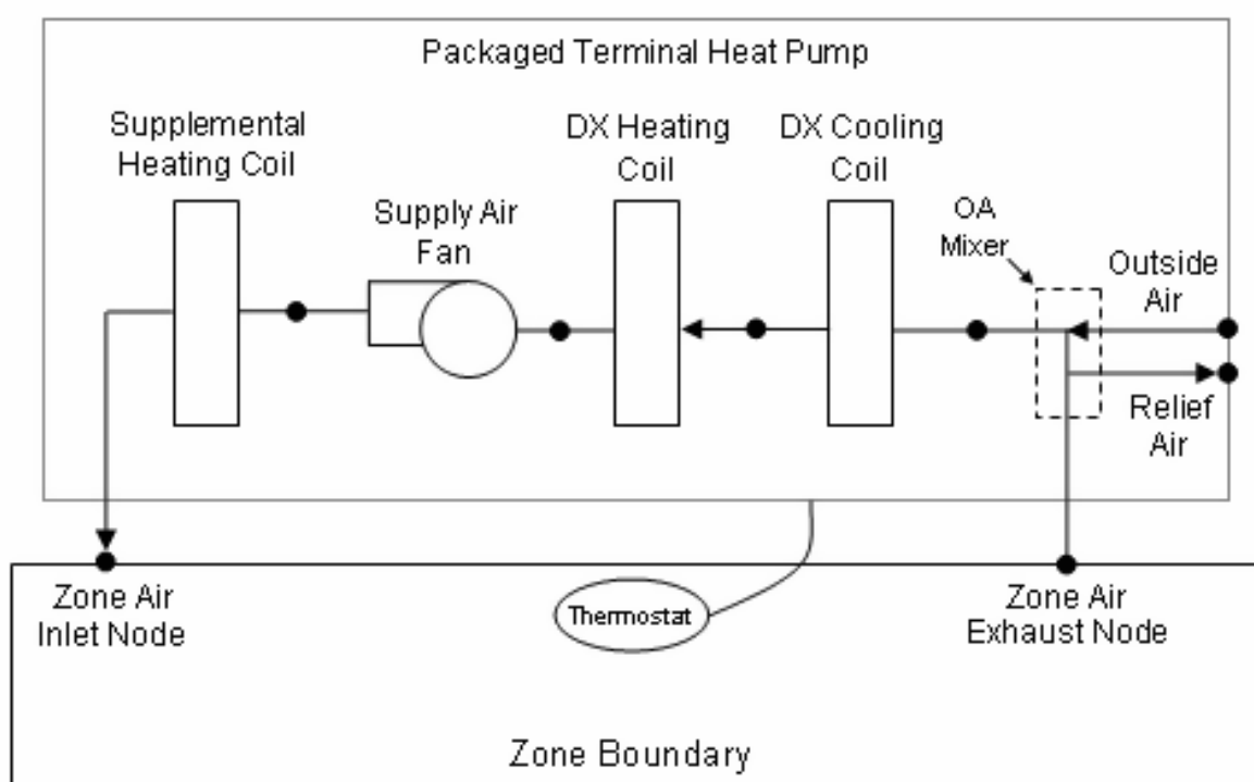
Figure 19.23: Schematic of a Packaged Terminal Heat Pump (Draw Through Fan Placement)
