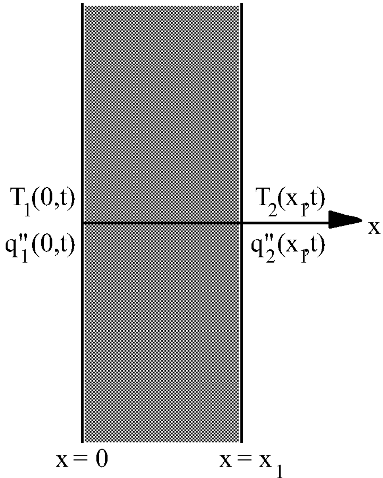
Figure 18.1: Single Layered Building Element
