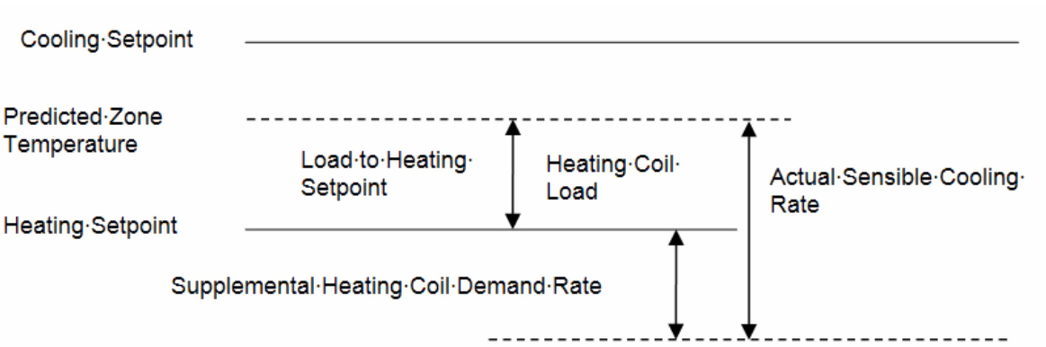
Figure 16.28: Supplemental heating coil load when predicted zone air temperature is above the heating Setpoint
