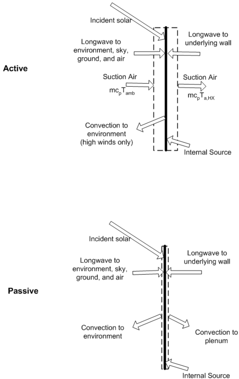
Figure 18.39: Transpired Collector Heat Balance
