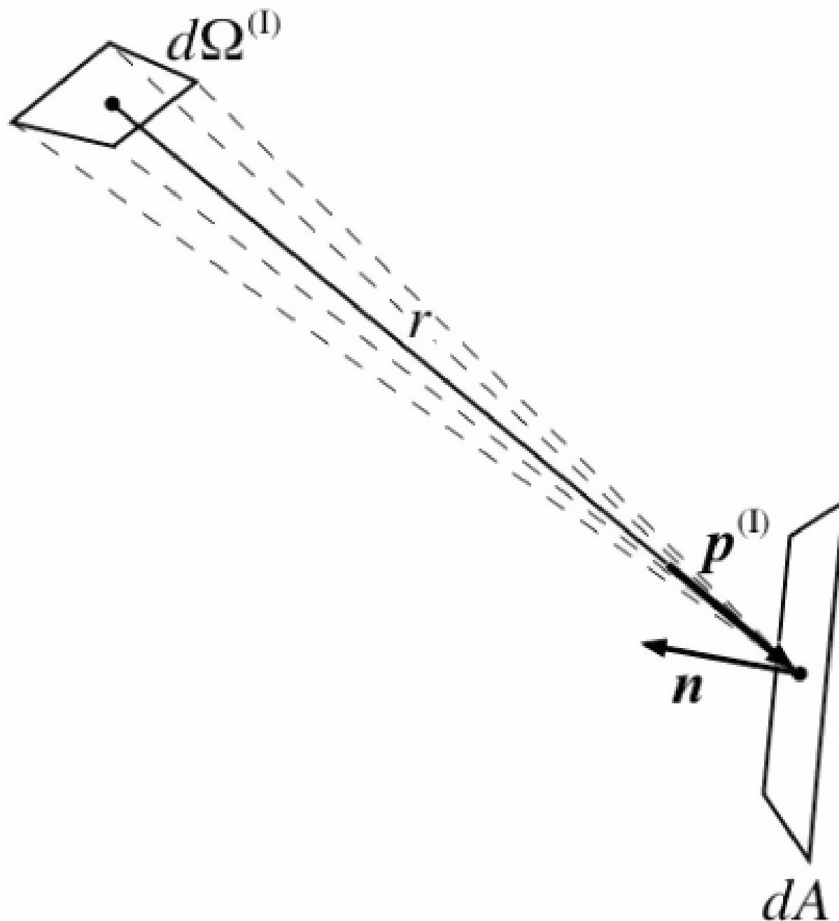
Figure 7.34: Irradiance geometry
