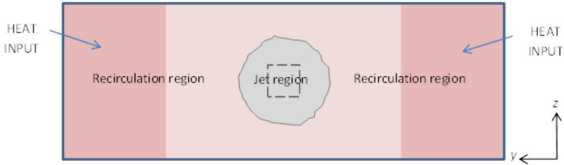
Figure 13.21: Jet and recirculation regions in typical vertical cross-section through room (y-z plane). Jet boundary occurs where jet velocity has fallen to 50% of centerline maximum. Remainder of cross-section is treated as recirculation. Volumetric heat sources are
