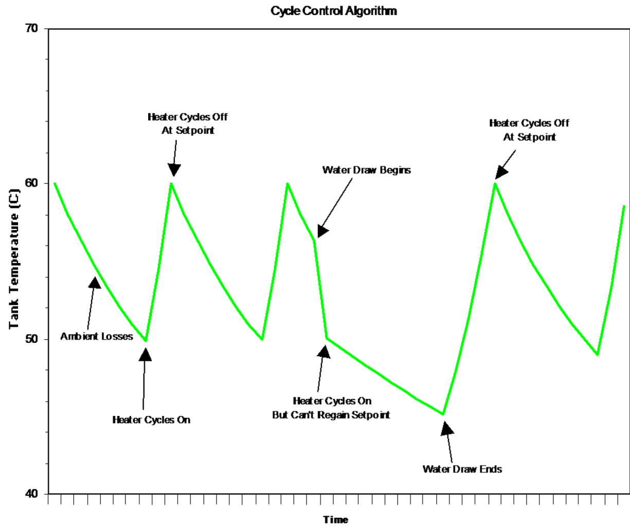
Figure 19.11: Water Heater Cycle Control Algorithm
