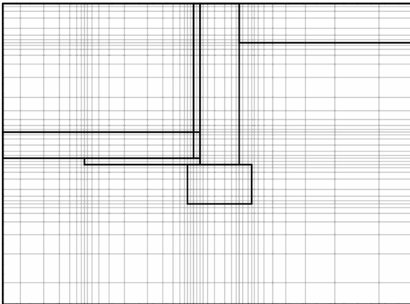
Figure 3.27: Example generated discretization near foundation perimeter
