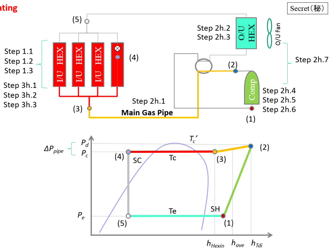
Figure 16.61: Schematic Pressure-Enthalpy Diagram for VRF Operation – Heating Mode
