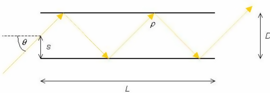
Figure 7.12: Discrete Ray in a Pipe
