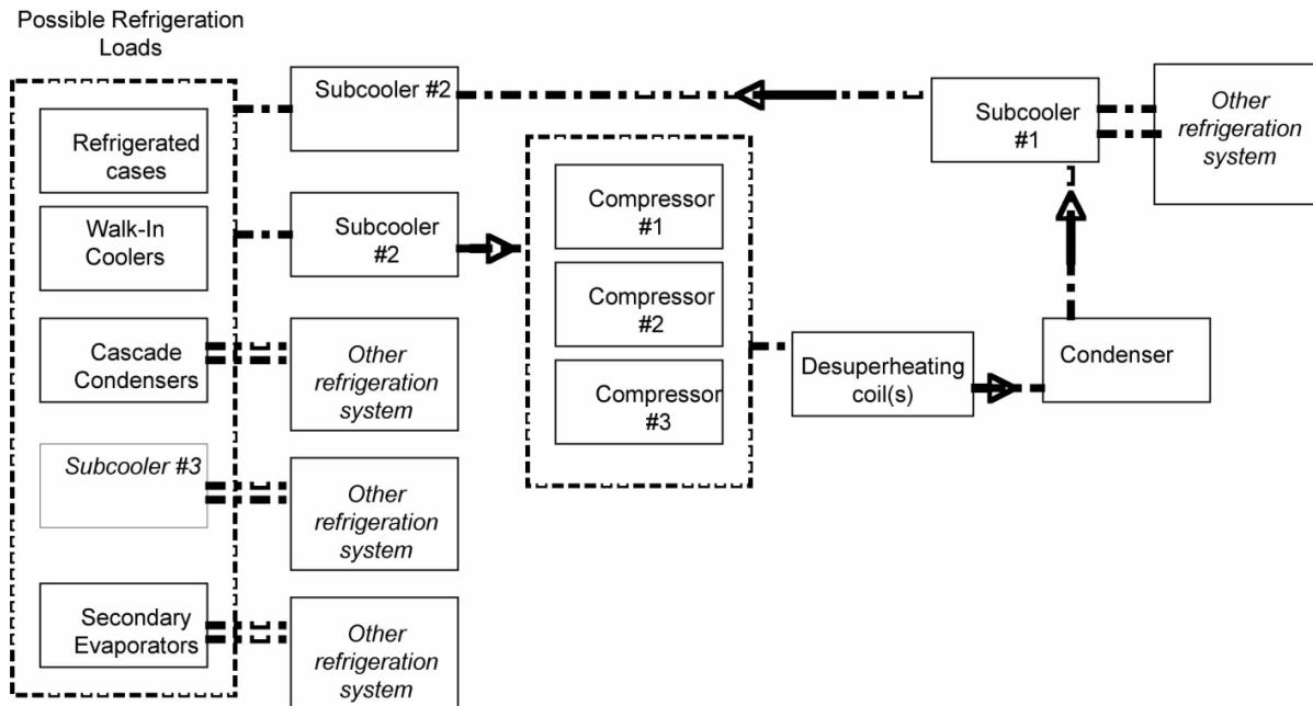
Figure 18.14: Typical Detailed Refrigeration System Equipment Schematic
