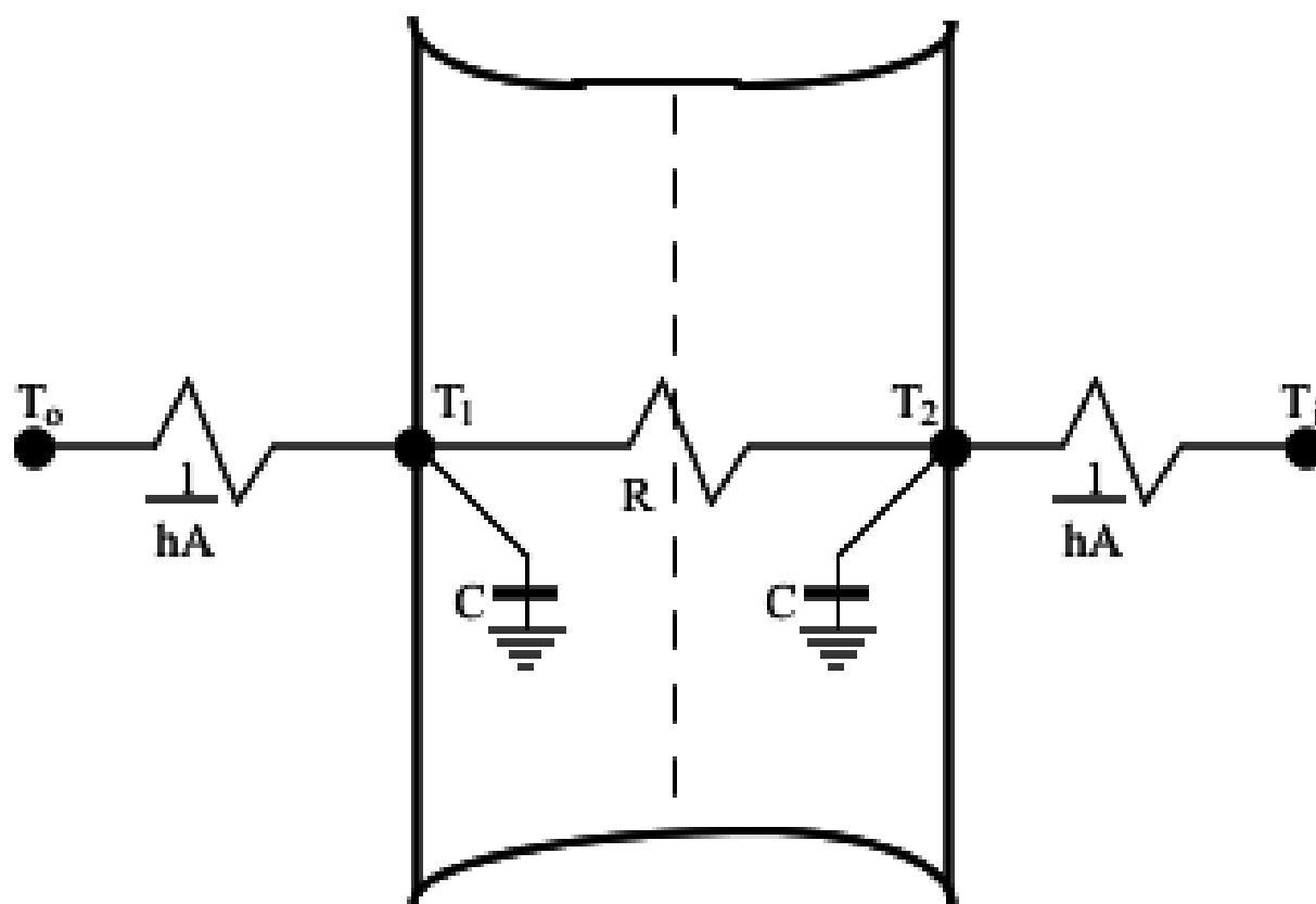
Figure 18.3: Two Node State Space Example
